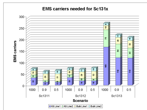
Figure 5: The Needed EMS Carriers for Scenarios Sc131x.
