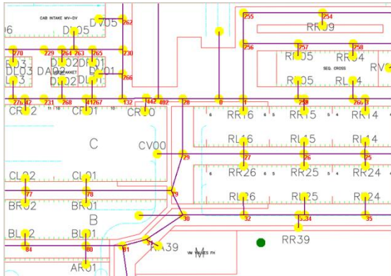
Figure 3: A Part of the Factory Layout of the Current Situation
