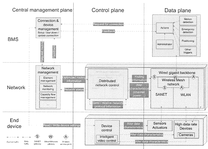
Fig. 2. Network architecture
