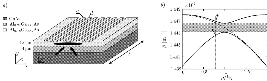
Fig. 1. a) Planar periodic structure: a=2\ \mu\text{m} , d=4\ \mu\text{m} . b) Band diagram based on Eq.1 in linear regime.
