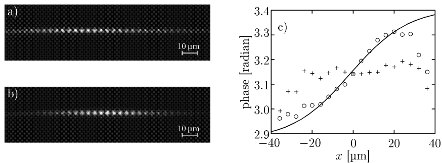
Fig. 3. Output intensity profile at low (a) and high (b) power when a stationary soliton is formed. c) Evolution of the phase of the intensity maxima towards the grating in the case of Fig.a) (+) and Fig.b) (o). The solid line shows the theoretical phase profile for a stationary gap soliton with \psi = 0.27 .
