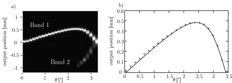
Fig. 2. a) Intensity profile at the output of a 16 mm long planar periodic waveguide for one incident beam. The angle \theta refers to the input angle in the waveguide. b) Lateral shift at the output for Bloch modes on the first band (+). The solid line shows the theoretical shift based on the diffraction relation plotted on Fig.1.b ( \kappa = 10300\ \text{m}^{-1} ).
