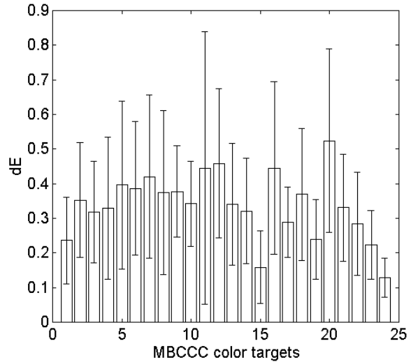
Fig. 3. The average medium-term precision of the MBCCC color targets. The error bars represent one sample standard deviation
