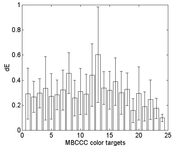
Fig. 4. The average long-term precision of the MBCCC color targets. The error bars represent one sample standard deviation
