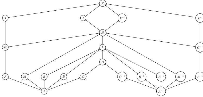
Fig. 2: Hasse diagram of thirteen neighborhood operators and their inverses
