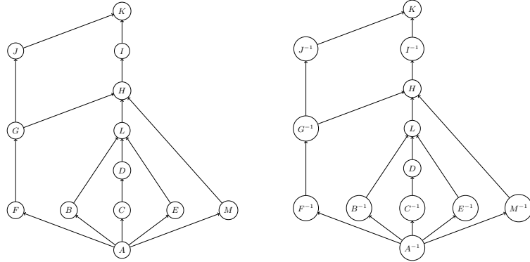
(a) Lattice of the neighborhood operators
