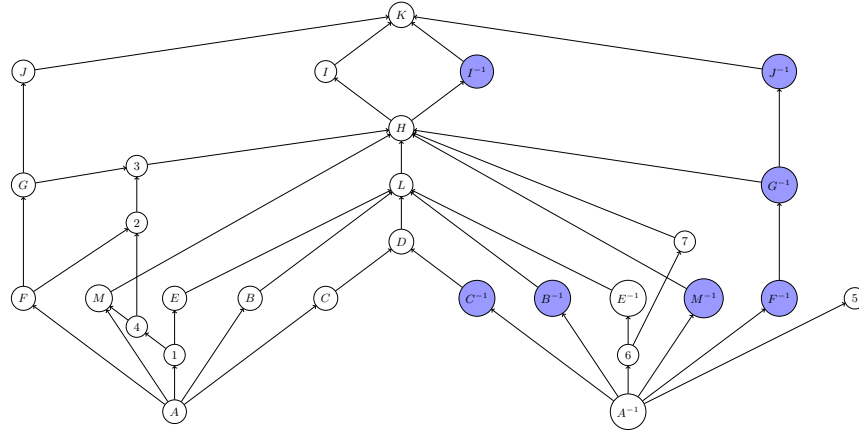
Fig. 3: Hasse diagram of twenty-nine upper approximation operators
