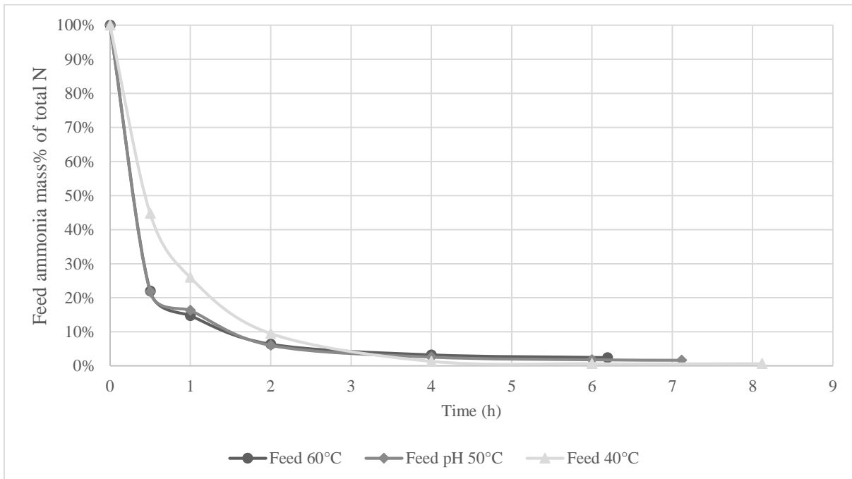
Figure 4: Feed mass percentage of total ammonia versus total time of the membrane distillation experiment. Urine of batch Hydro-01 was used, with a feed pH of 10.5. The membrane used in this series of experiments came from a single sheet of S02 membrane.
