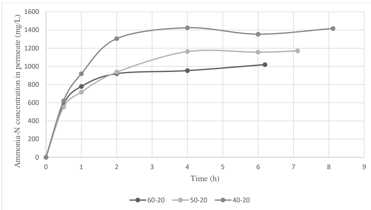
Figure 5: Concentration of ammonia in the acidified permeate. Urine of batch Hydro-01 was used, with a feed pH of 10.5. The membrane used in this series of experiments came from a single sheet of S02 membrane.
