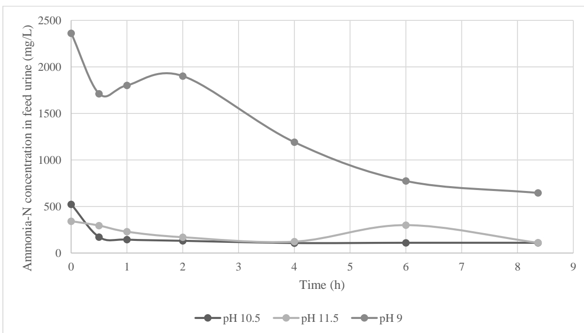
Figure 3: Concentration of ammonia in the feed urine. Urine of batch Hydro-02 was used, with respective feed and permeate temperatures of 50 and 20°C. The membrane used in this series of experiments came from a single sheet of NS02 membrane.
