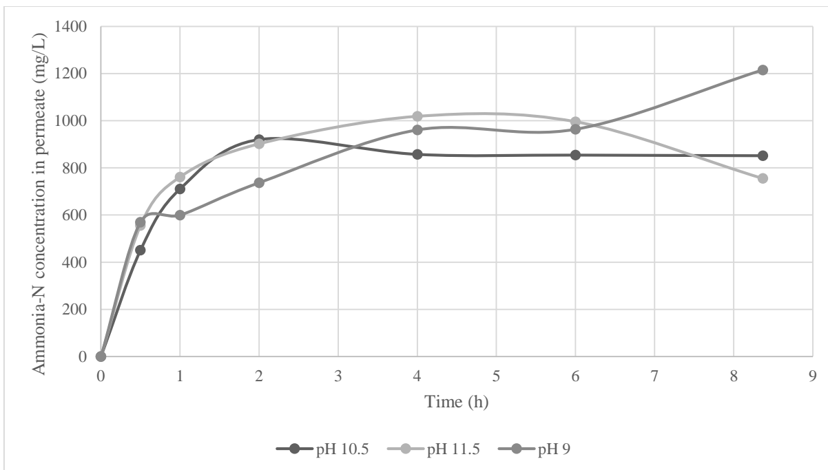
Figure 2: Concentration of ammonia in the acidified permeate. Urine of batch Hydro-02 was used, with respective feed and permeate temperatures of 50 and 20°C. The membrane used in this series of experiments came from a single sheet of NS02 membrane.
