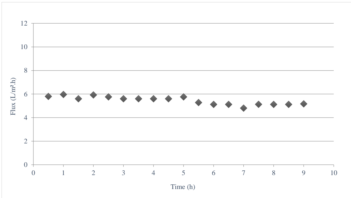
Figure 7: Water flux in a membrane distillation experiment using batch FRESH-01 urine. T_{\text{feed}}=50^{\circ}\text{C} , T_{\text{permeate}}=20^{\circ}\text{C} , pH unadjusted (pH 7). Experiments were run to a concentration factor of 3, the membrane used is a NS01 membrane.
