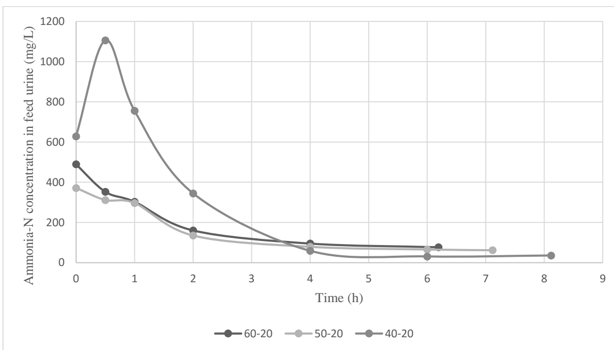
Figure 6: Concentration of ammonia in the feed urine. Urine of batch Hydro-01 was used, with a feed pH of 10.5. The membrane used in this series of experiments came from a single sheet of S02 membrane.
