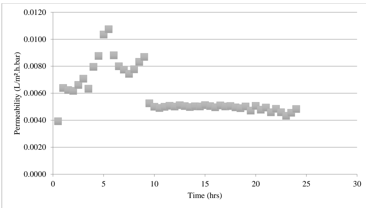
Figure 10: Long-term membrane distillation experiment, using 2 L of batch Fresh-01 urine. T_{\text{feed}}=50^{\circ}\text{C} , T_{\text{permeate}}=20^{\circ}\text{C} . The pH was unadjusted at 7. Membrane used: S02.
