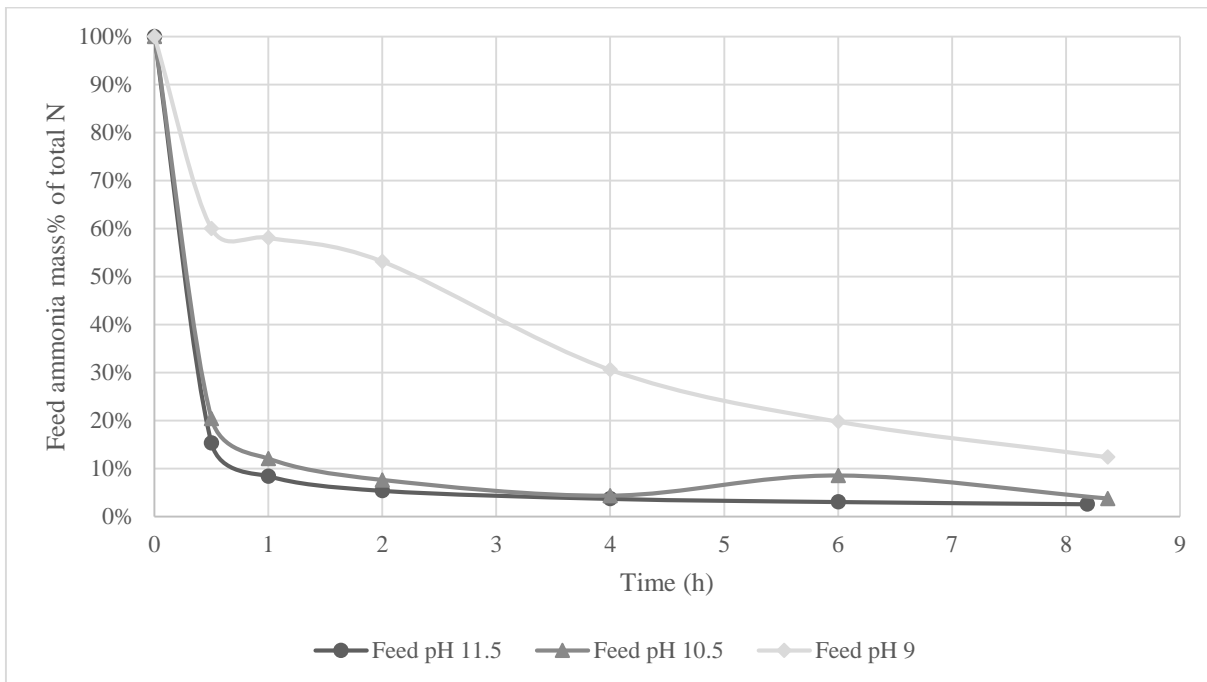
Figure 1: Feed mass percentage of total ammonia versus total time of the membrane distillation experiment. Urine of batch Hydro-02 was used, with respective feed and permeate temperatures of 50 and 20°C. The membrane used in this series of experiments came from a single sheet of NS02 membrane.
