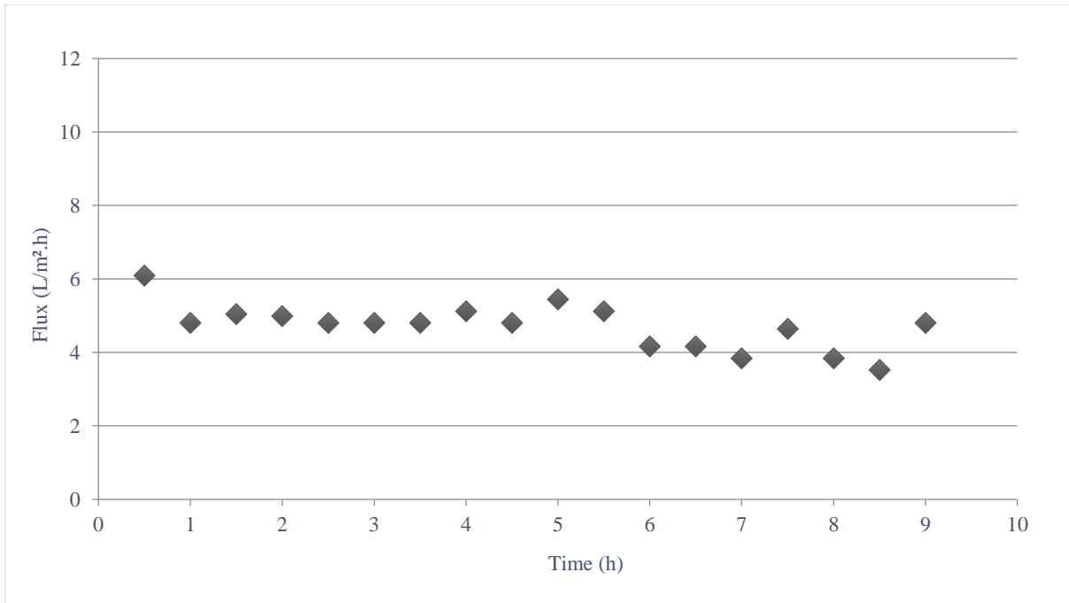
Figure 8: Water flux in a membrane distillation experiment using batch HYDRO-02 urine. ( T_{\text{feed}}=50^{\circ}\text{C} , T_{\text{permeate}}=20^{\circ}\text{C} , pH adjusted to 12). Experiments were run to a concentration factor of 3, the membrane used is a NS01 membrane.
