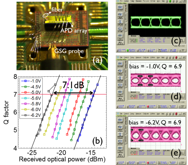
Figure 4. (a) Ge waveguide APD array, wire-bonded to a CMOS TIA array. (b) Measured electrical Q factor vs. received optical power and APD bias voltages. (c) 10Gb/s reference optical eye diagram. (d) 10Gb/s eye diagram at -1.0V. (e) 10Gb/s eye diagram at -6.2V.
