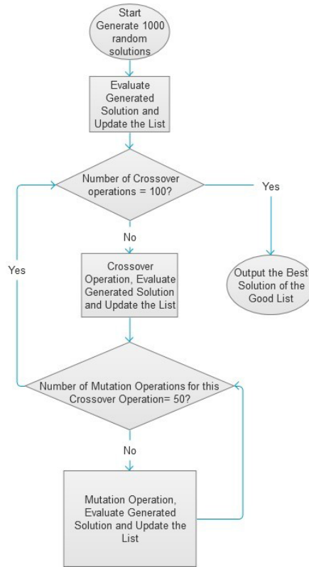
Fig. 2 Flow Chart of Our Algorithm
