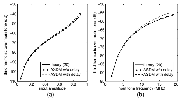
Fig. 5. Comparing the distortion of two equivalent second order ASDMs with theory.
