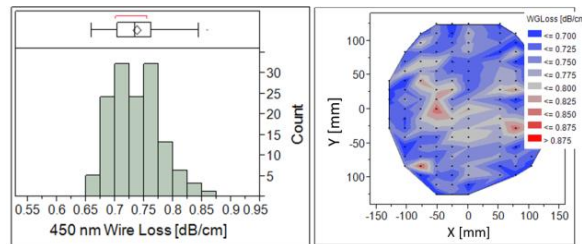
Fig. 3. Within wafer propagation loss uniformity of a 450nm wire waveguide.
