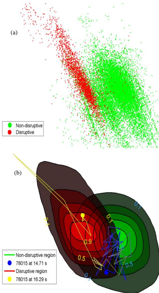
Figure 2: Two-dimensional projections from JET disruption data (a). Disruptive and non-disruptive clusters of data points are mapped using LMDS with 10 landmark points. (b). Density contours for the data points belonging to disruptive and non-disruptive clusters are drawn. The numbers give a qualitative measure of the degree of the disruptiveness of the region. A trajectory for pulse 78015 is also traced.
