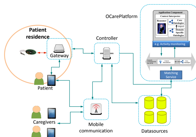
Figure 1: Architecture of the OCareCloudS system
