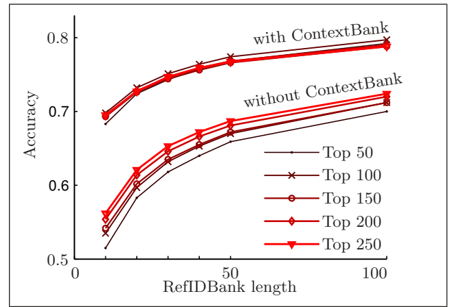
Figure 4: Influence of context on accuracy for 5 different dataset sizes
