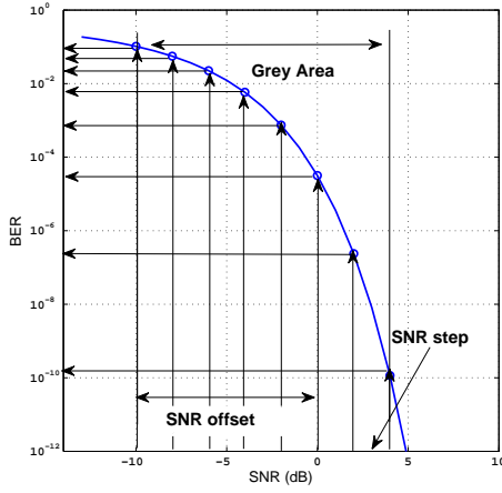
Fig. 15. Quantized BER curve
