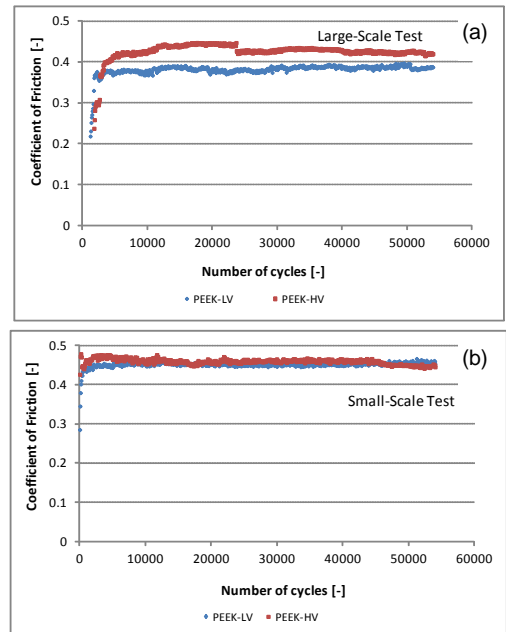
Figure 3. Comparison of on-line measurements of the coefficient of friction between (a) large-scale and (b) small-scale test at a contact pressure of 10 MPa and sliding velocity of 20 mm/s.
