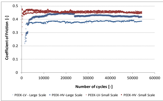
Figure 4. Comparison of on-line measurements of the coefficient of friction all together large-scale and small-scale test at a contact pressure of 10 MPa, and sliding velocity of 20 mm/s.
