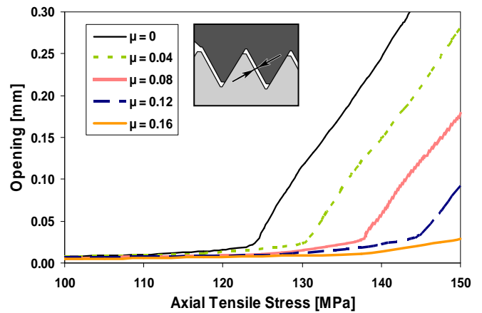
Fig. 10: Influence of the coefficient of friction on the thread opening
