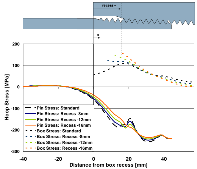
Fig. 16: Hoop stress at the inside wall of the pin and the outside wall of the box at make-up for different values of the box recess length.
