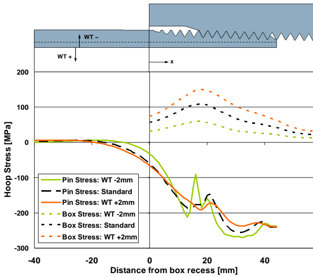
Fig. 14: Hoop stress at the inside wall of the pin and the outside wall of the box at make-up for different values for the pin wall thickness.
