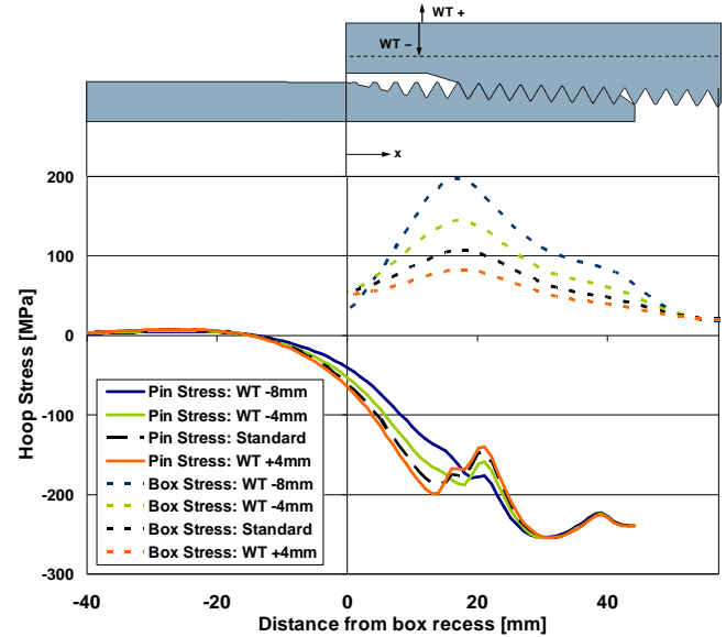
Fig. 12: Hoop stress at the inside wall of the pin and the outside wall of the box at make-up for different values for the box wall thickness.
