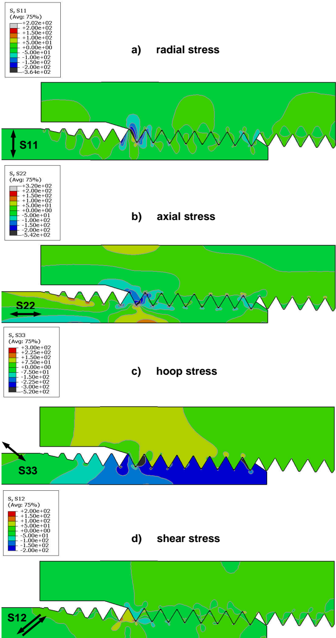
Fig. 7: Stress components at make-up
