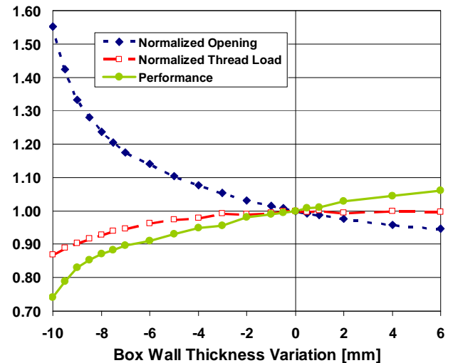
Fig. 13: Influence of the box wall thickness on the connection parameters
