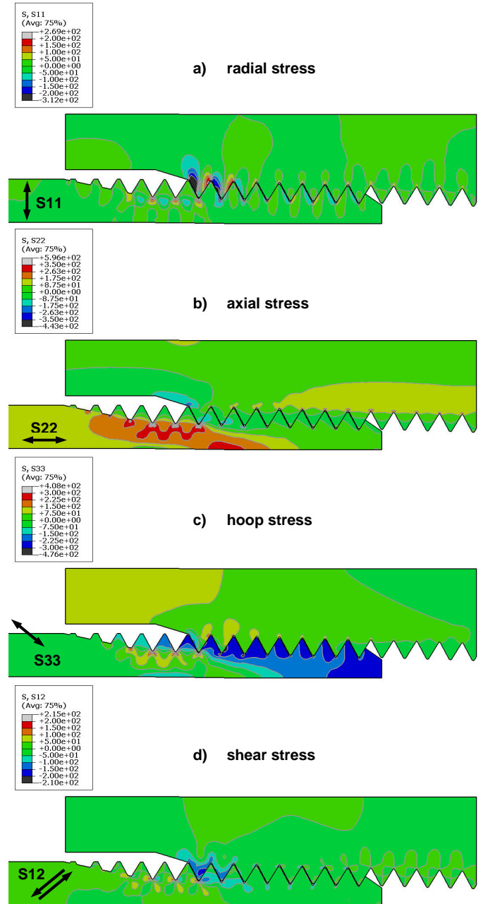
Fig. 8: Stress components with an additional axial load of 150 MPa
