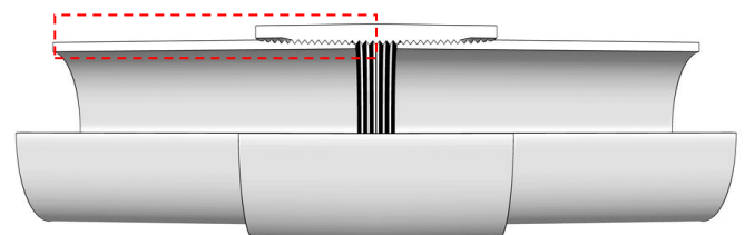
Fig. 2: Section view of an API Line Pipe Connection
