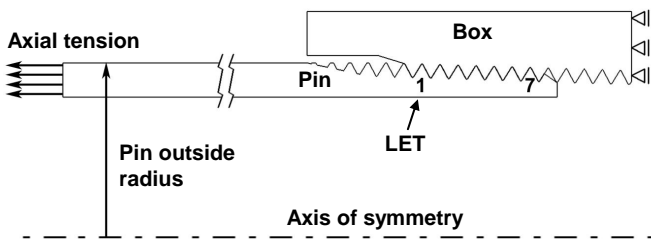
Fig. 3: 2D axisymmetric model of the API Line Pipe connection
