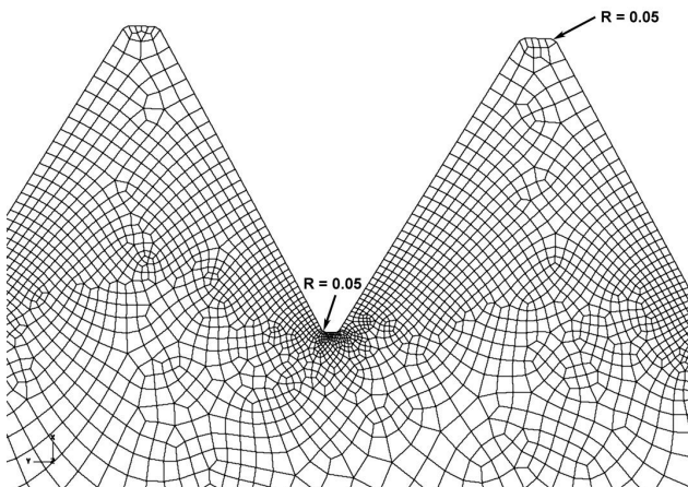
Fig. 5: Detailed mesh around thread root of the pin
