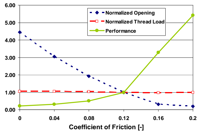
Fig. 11: Influence of the coefficient of friction on the connection parameters
