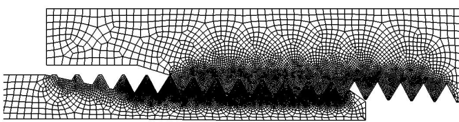
Fig. 4: Mesh of the FE model
