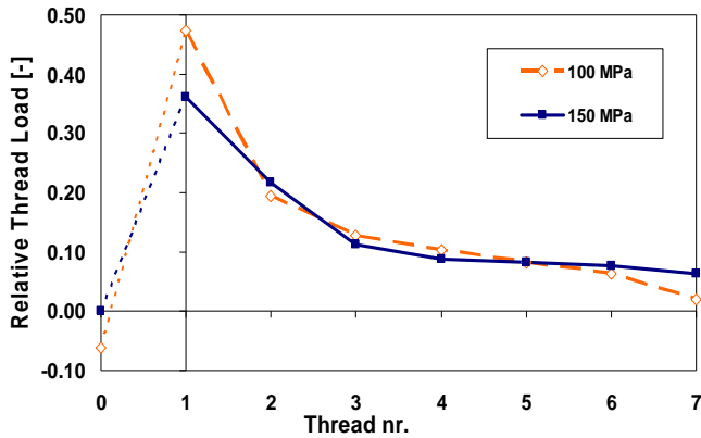
Fig. 9: Thread load distribution (numbering as in Fig. 3)
