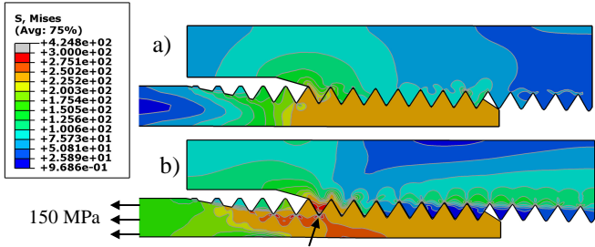
Fig. 6: von Mises stress distribution a) at make-up; b) with an external axial tensile stress of 150 MPa
