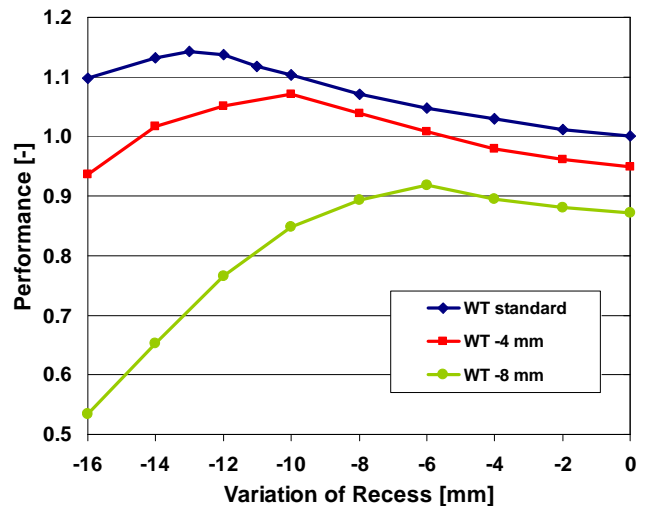
Fig. 17: Influence of the box recess length and wall thickness on the connection performance
