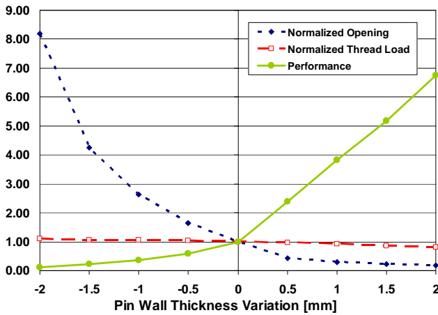
Fig. 15: Influence of the pin wall thickness on the connection parameters
