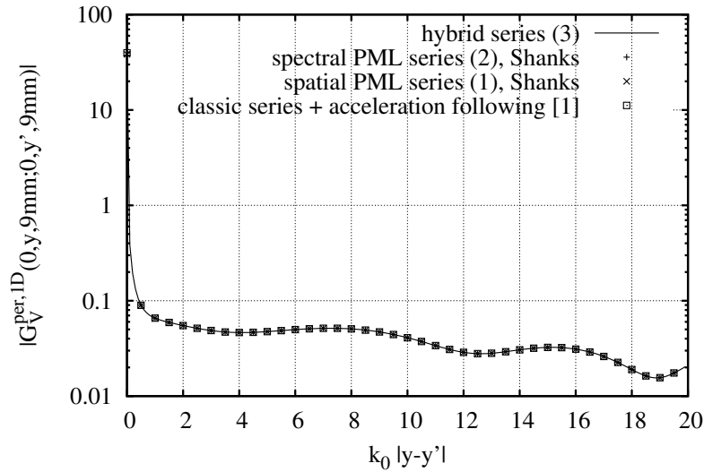
Figure 2: 1D periodic 3D Green's function |G_V^{\text{per},1D}(x, 0, 9 \text{ mm}; x', 0, 9 \text{ mm})| .
