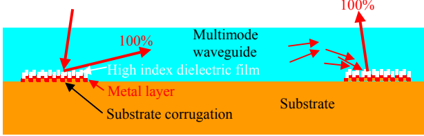
Fig.2: Experimental simulation of an optical interconnect input/output multimode waveguide grating coupler
