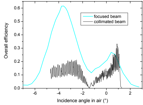
Fig.3: Overall efficiency measured with a focused and a collimated beam at 850 nm wavelength under TE polarization
