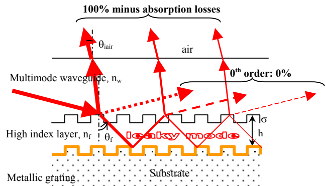
Fig. 1. Outcoupling resonant grating and scheme of the leaky mode mediated destructive interference of 0 th order reflection.
