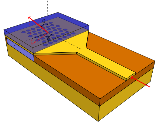
Fig. 1. Light is coupled out as a Lorentzian beam with inclination \theta and azimuth \phi .
