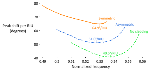
Fig. 3. Sensitivity for various cladding configurations. As expected, the symmetric cladding case is the most sensitive.
