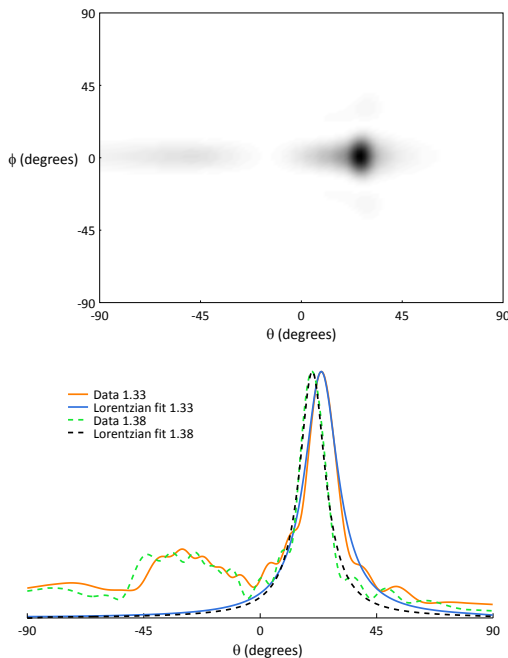
Fig. 2. Spectral image of outcoupled light (top) with cross-section at \phi=0^\circ (bottom) where the Lorentzian shape can be distinguished. The refractive index of the cladding layers above and below the PhC as well as that of the holes all vary ( symmetric cladding type). The normalised frequency is 0.53488.
