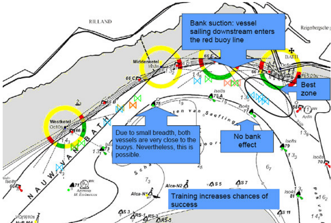
Figure 8: Evaluation of the encounter locations for the Bend of Bath at maximum ebb current
