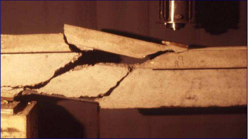
Fig. 3. Shear failure of a concrete beam, without stirrups with T-shaped cross-section
