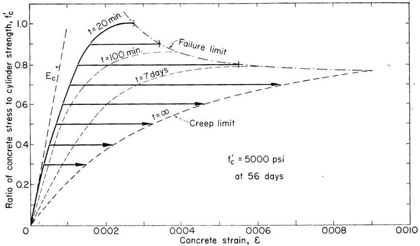
Fig. 1. Influence of sustained loading on the compressive strength of concrete according to Rüsçh [1] (age at loading : 28 days)
