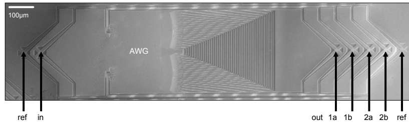
Fig. 3. SEM of fabricated duplexer. The outermost fiber couplers are directly connected and are used for as alignment and reference. The AWG has a 600 \times 350 \mu\text{m}^2 footprint. The two outputs for each wavelength band are not grouped but characterised individually.
