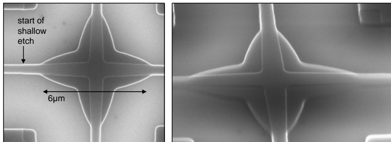
Fig. 3. Fabricated crossings. The shallow etch region can be clearly discerned.
