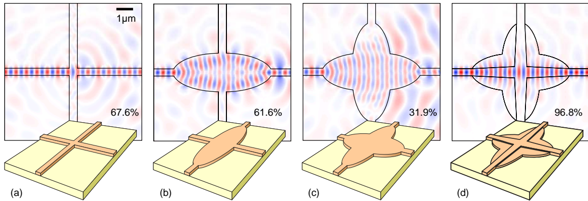
Fig. 2. 2-D simulations of different waveguide crossings. (a) direct crossing, (b) two-fold symmetric elliptical crossing as presented in [2], but with a length of 6 \mu\text{m} , (c) elliptical crossing from [2], but with a 6 \mu\text{m} length, (d) crossing with deep and shallow etch.
