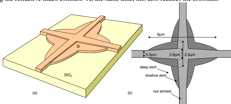
Fig. 1. Waveguide crossing with expanded waveguides and double etch.
