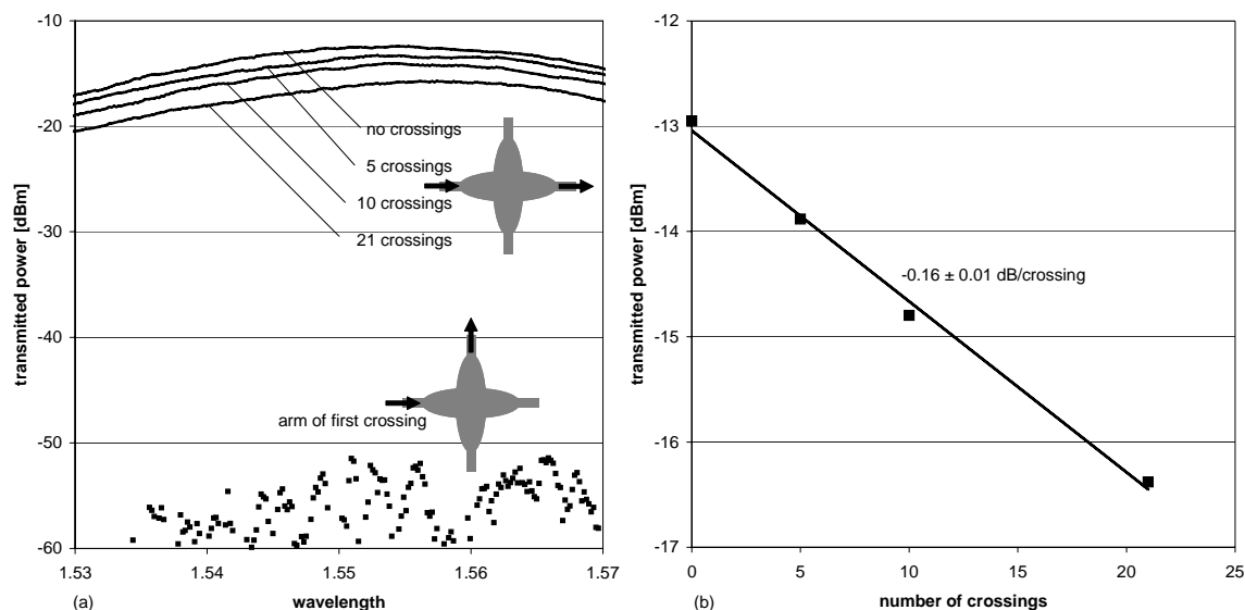
Fig. 4. Transmission measurements on multiple waveguide crossings. (a) transmission spectrum for 0, 5, 10 and 21 crossings. The parabolic Gaussian spectrum is characteristic for grating fiber couplers [7]. (b) fitted loss per crossing at a wavelength of 1550nm.
