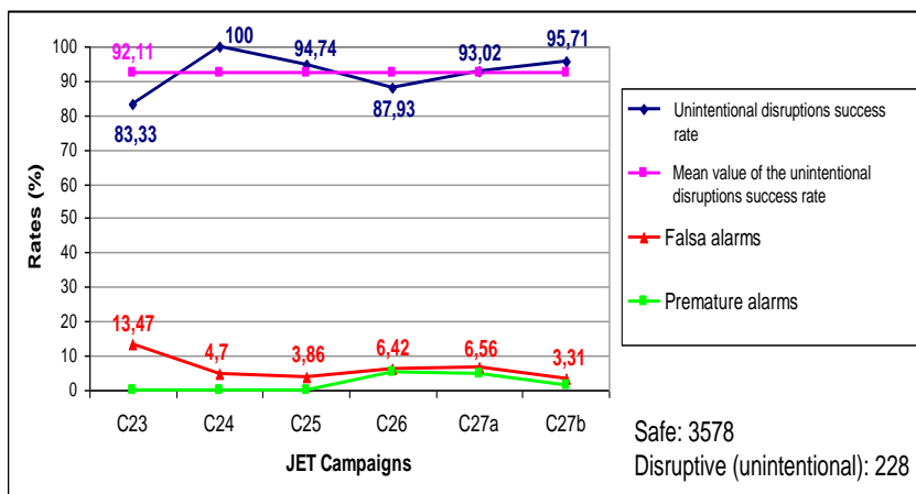
Figure 2 Success rate of APODIS for various JET campaigns with the Carbon wall in absolutely realistic real time conditions.
