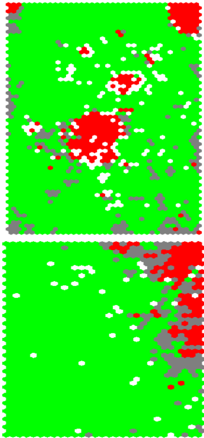
Figure 5 Top: SOM map of disruptive and safe discharges for JET: Bottom: SOM map of disruptive and safe discharges for AUG [10]. The colour code is: green safe clusters, red disruptive clusters, gray mixed clusters and white empty clusters. Both databases contain hundreds of thousands of points.
