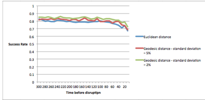
Figure 3: The overall success rate for the clustering based on the Euclidean and Geodesic distances.
