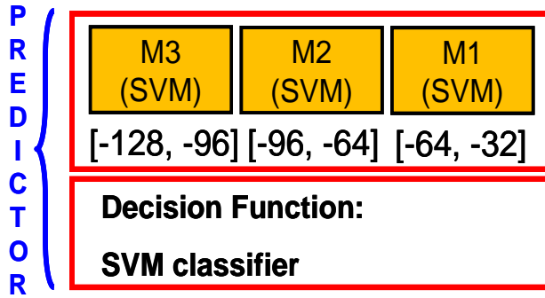
Figure 1: Architecture of the predictor APODIS. M1, M2 and M3 are three SVM classifiers analyzing three subsequent windows of data (times in ms). The decision function is implemented by an additional independent SVM.
