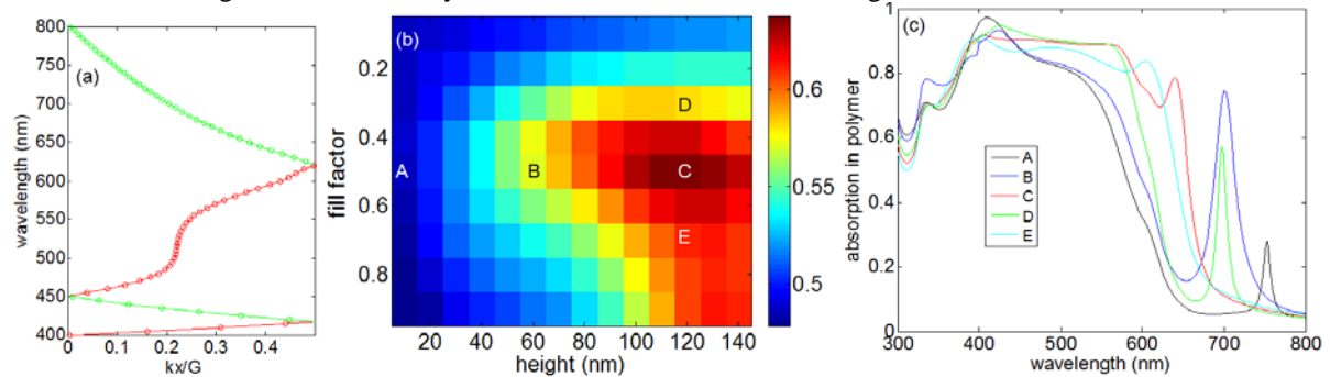
Fig. 2. (a) Dispersion diagram of SPP mode at a flat polymer-silver interface folded with 400nm grating period, where G is the reciprocal lattice vector. (b) Dependence of integrated absorption efficiency in the 300-800nm region. (c) TM polarization absorption spectrum at different points in (b).
