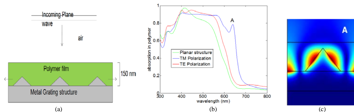
Fig. 1. (a) The simulated system, a plane wave incoming at normal incidence to the solar cell structure. (b) Polymer absorption spectrum for the planar and patterned device, respectively. The patterned device has a period of 400nm with fill factor 0.5 and triangle height 120nm. (c) Plot of the norm of the magnetic field profile for the TM polarization input at 640nm wavelength.
