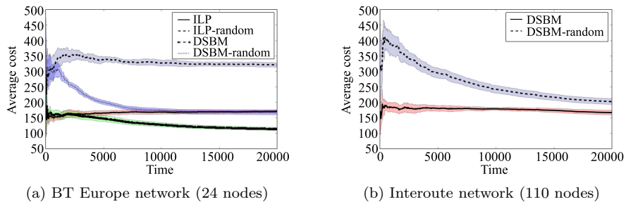
Figure 6: Average cost of accepting requests over time. The shaded background behind each curve represents the 95% confidence interval on the reported average values.
