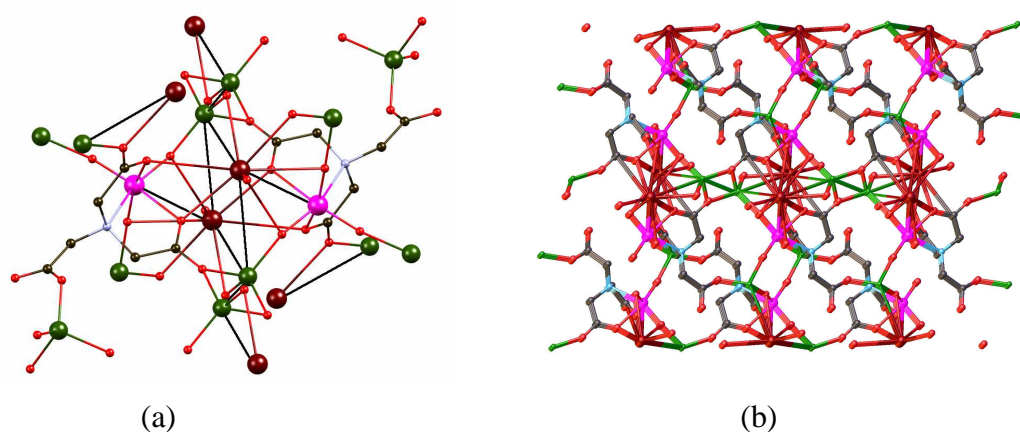
Fig. 4 (a) Ball and stick model showing part of the polymeric structure. Metal-metal interactions are shown by black lines. (b) View along crystallographic b axis of the 3D network of 1 . Color Code: Mo: pink, Li: green, K: dark brown, O: red, N: light blue, C: black, H atoms are not shown for clarity.
