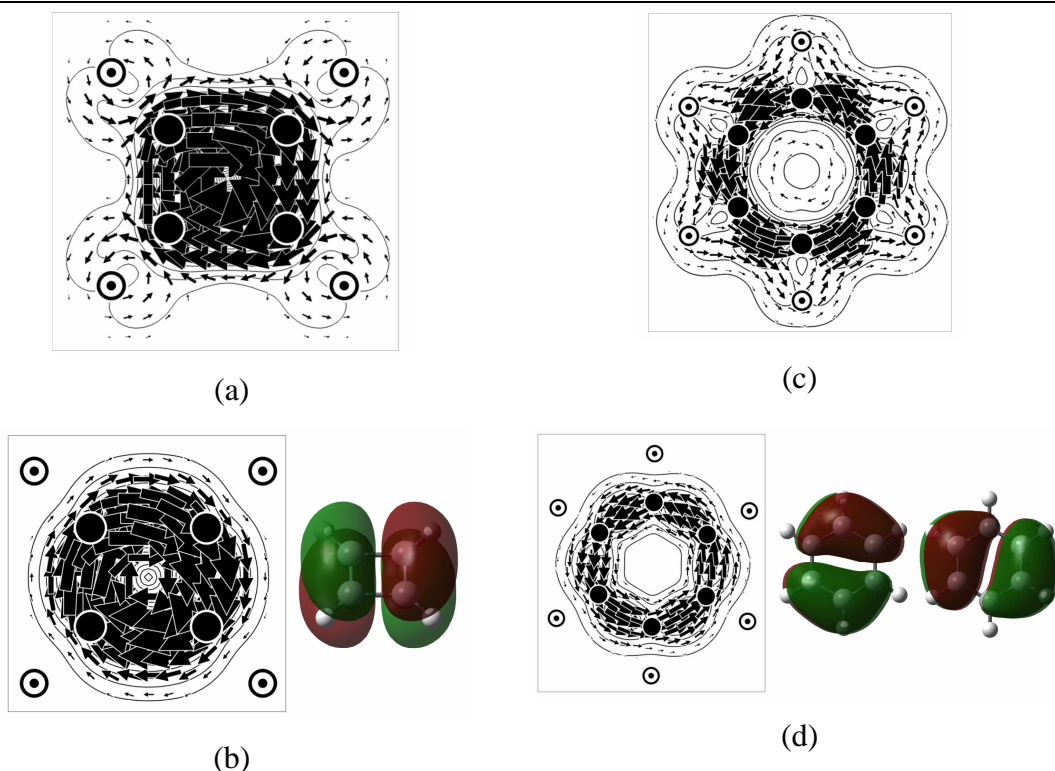
Fig. 18 Current density maps of cyclobutadiene 1 Å above the molecular plane: a) total current density b) HOMO current density. Current density maps of benzene 1 Å above the molecular plane: c) total current density d) doubly degenerate HOMO current density. H and C atoms are represented by dotted and filled circles, respectively.
