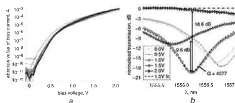
Fig. 2 Static characteristics of device
