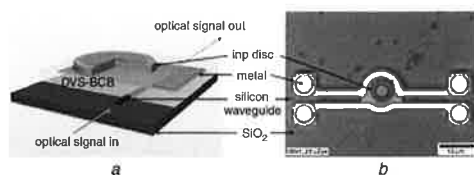
Fig. 1 Device structure of heterogeneously integrated InP microdisc modulator; silicon waveguide and silicon dioxide ( \text{SiO}_2 ) cladding are indicated
