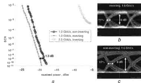
Fig. 3 Dynamic measurements of InP microdisc modulator
