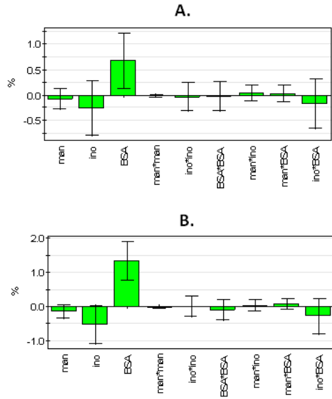
Fig. 2. Huyge Main experiments: coefficient plots of residual moisture content (A) and hygroscopicity (B) responses (man = mannitol; ino= inositol; BSA = Bovine Serum Albumin). Note the significant positive effect of BSA on the residual moisture content and hygroscopicity.
