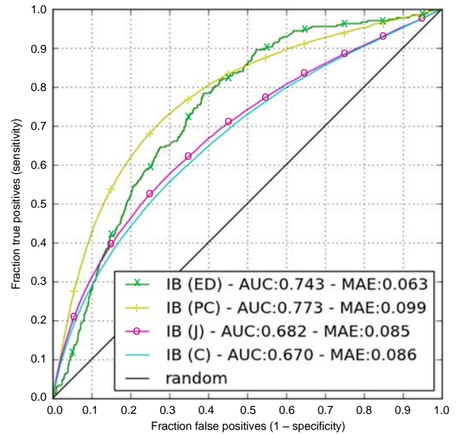
Fig. 5. ROC curve and MAE for item-based CF on implicit data with userCO=5 and topN=60.
