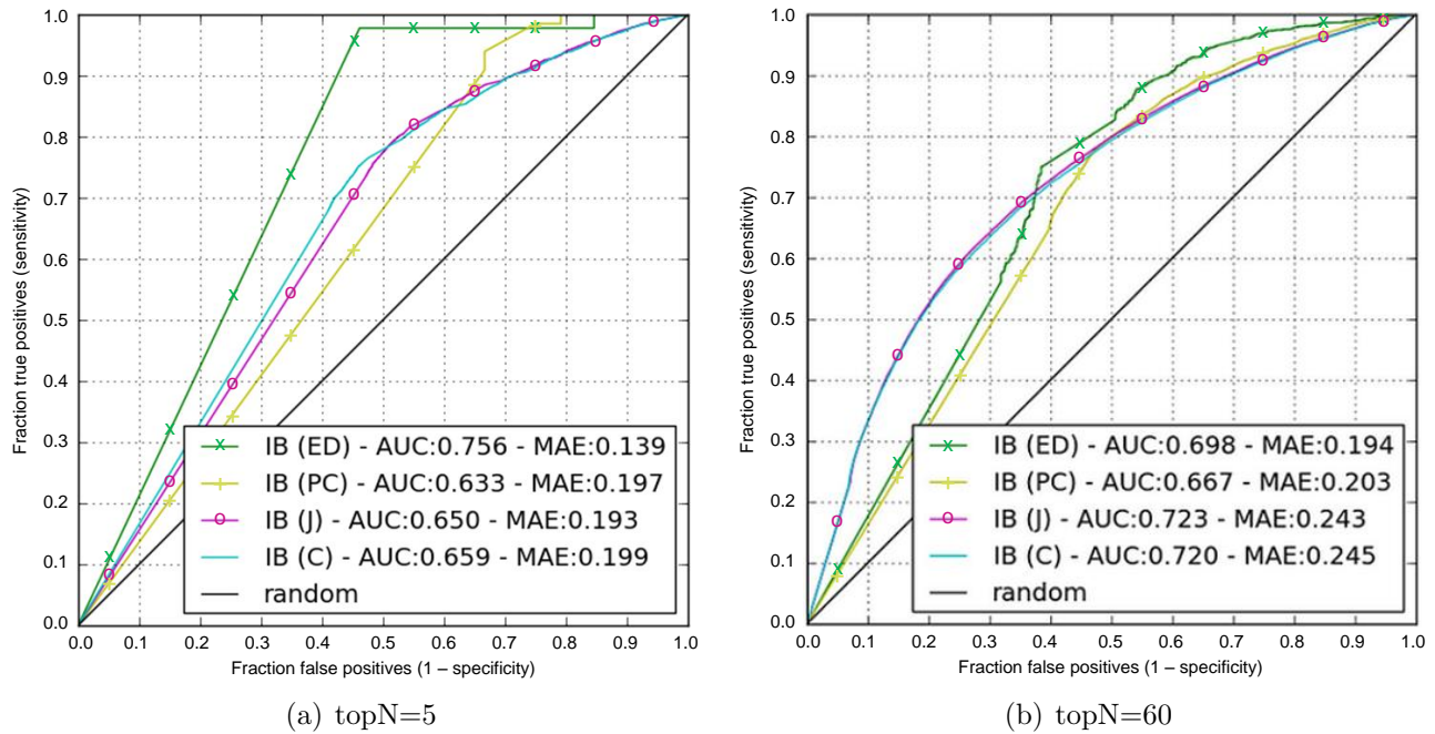
Fig. 4. ROC curve and MAE for item-based CF on explicit data with userCO=5.
