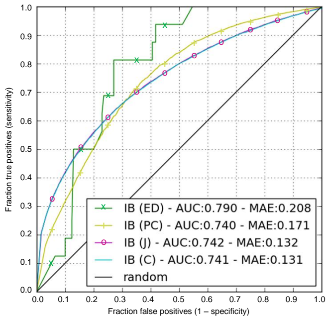
Fig. 6. ROC curve and MAE for combined item-based CF with a 1-1 ratio for the implicit and explicit ratings. userCO=10 and topN=10.
