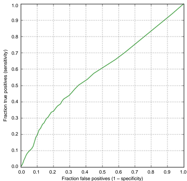
Fig. 2. ROC curve content-based CF on the explicit dataset with userCO=20 and topN=5.
