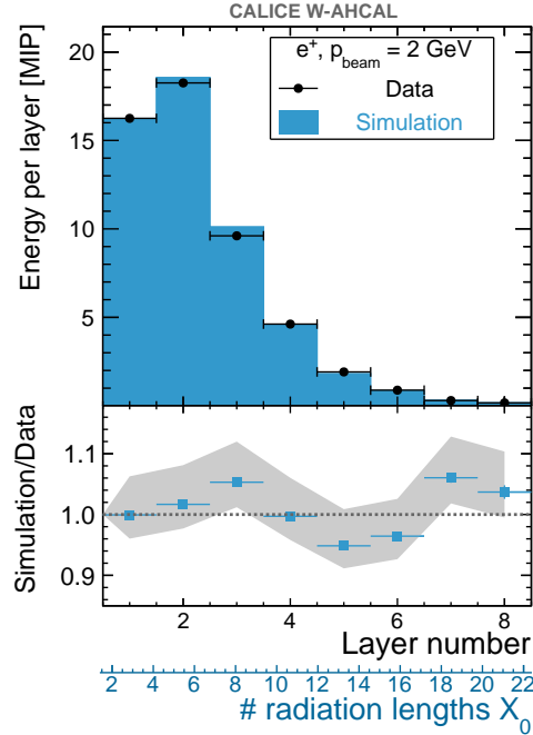
Figure 9. Longitudinal shower profile for 2 GeV e^+ : comparison of data with simulation. In the bottom part of the figure the ratio between the simulation and the data is shown. The grey band shows the overall uncertainty.
