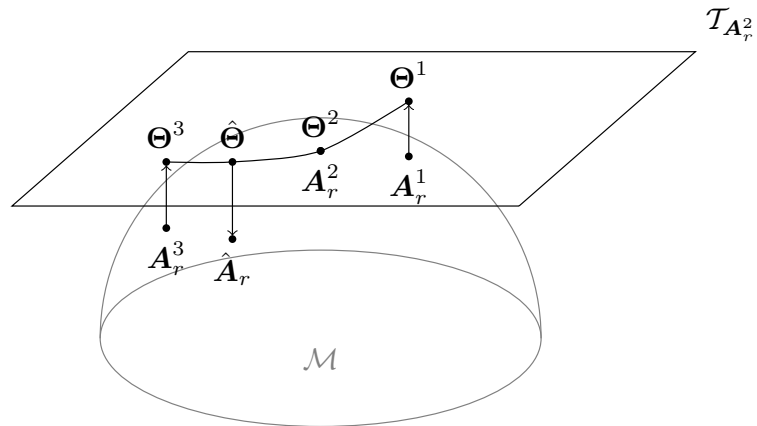
Figure 1. Representation of the Riemannian manifold \mathcal{M} and the space \mathcal{T}_{A_r^2} , tangent to the manifold at A_r^2 . The matrices A_r^1 and A_r^3 are mapped to \Theta^1 and \Theta^3 in \mathcal{T}_{A_r^2} with the logarithmic mapping \text{Log}_{A_r^2} . Subsequently, the interpolation of their images \Theta^i is performed in the tangent space and the result \hat{\Theta} is mapped to \hat{A}_r on the manifold with the exponential mapping \text{Exp}_{A_r^2} . Adapted from [42].
