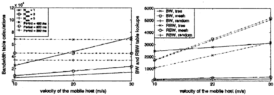
Fig. 4. Average number of Bandwidth table calculations (left figure) for the tree topology. The results for the mesh and random topology are very similar. Average number of lookups for the Bandwidth (BW) and Reuse-Bandwidth (RBW) table (right figure)
