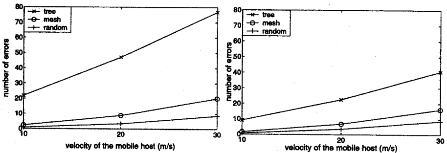
Fig. 6. The average number of errors per simulation. For the left figure, all access routers start to send beacons at 0.5 s. For the right figure, the start times for access router 1; ... ; 8 are given by (0.125 s; 0.75 s; 0.375 s; 0.0 s; 0.5 s; 0.875 s; 0.25 s; 0.625 s)
