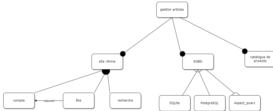
FIGURE 2.2 – Diagramme de features
