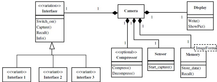
FIGURE 2.1 – Diagramme de classes
