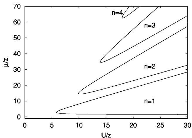
FIG. 1. The mean-field phase diagram in the units we adopt throughout the paper. The Mott lobes are indicated and surrounded by a superfluid.
