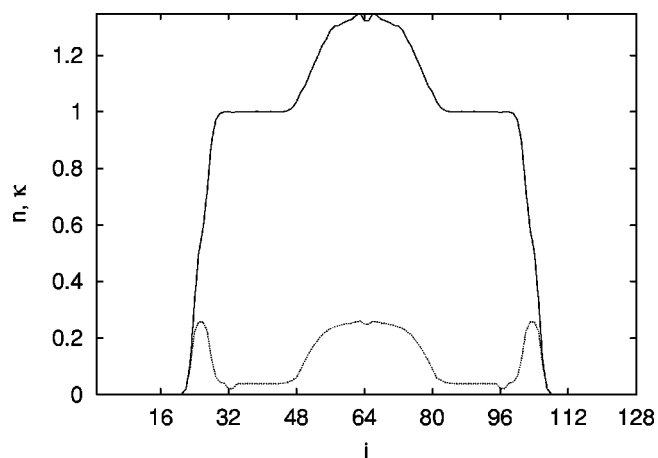
FIG. 8. Profile of the local density n (solid line) and local compressibility \kappa (dashed line) along the sites for U/2=7.1, \mu/2=6.1, L=128, v_c=0.008 , confirming again the result of Ref. [23].
