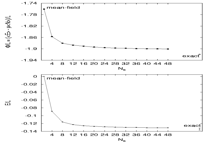
FIG. 3. Upper: The system is variational in the average grand-canonical potential per site \Phi/L = (\langle E \rangle - \mu \langle N \rangle) / L . As the number of kept states N_s is increased, the grand-canonical potential decreases. The full line is a guide to the eye. The parameters are chosen such that the system is near a generic phase transition on the SF side ( U=4, \mu=1, L=1024 ). This corresponds to the worst case scenario for our method. The mean-field ( N_s=1 ) and exact (corresponding to N_s=\infty ) results are indicated. Lower: The exponential convergence of the energy is shown. The system is deep in the Mott phase with parameters U=30, \mu=16 , and L=1024 .
