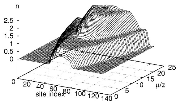
FIG. 7. Profile of the local density n along the sites and as a function of the chemical potential \mu . The on-site repulsion is U/2 = 7.1 . Above a certain value of \mu we see the emergence of a plateau ( n=1 ), and when the total number of particles is even more increased, we see the reemergence of a compressible region. This happens first around the center and continues to exist till a plateau with n=2 is reached. These results confirm the result of Ref. [23].
