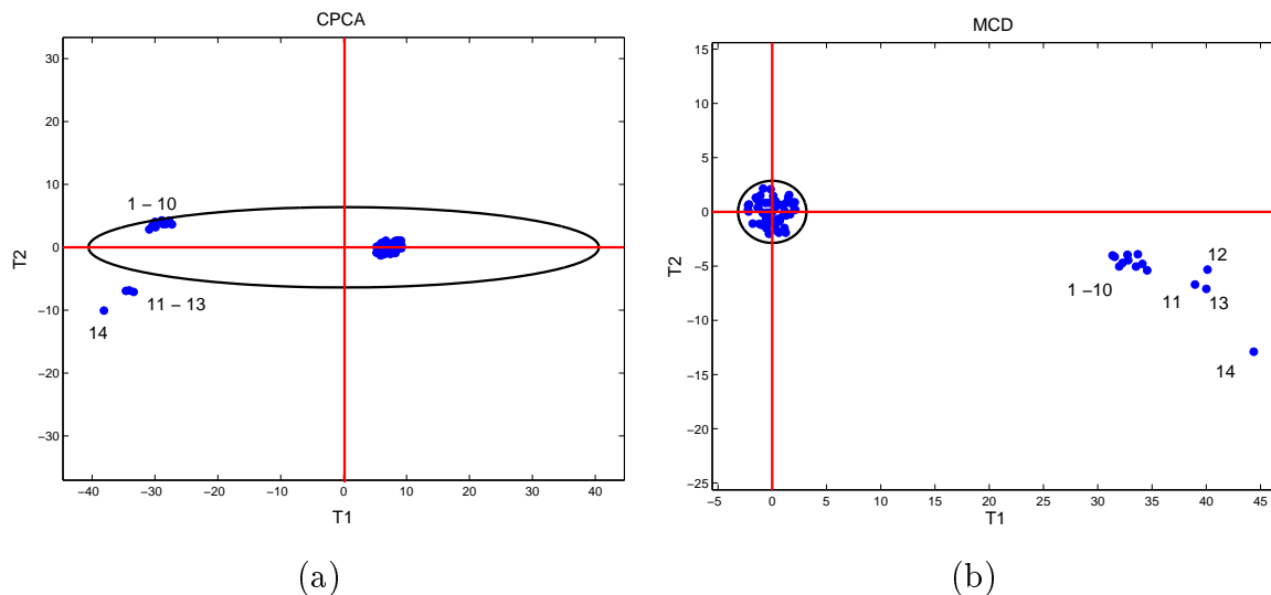
Figure 10: Score plot and 97.5% tolerance ellipse of the Hawkins-Bradru-Kass data obtained with (a) CPCA; (b) MCD.
