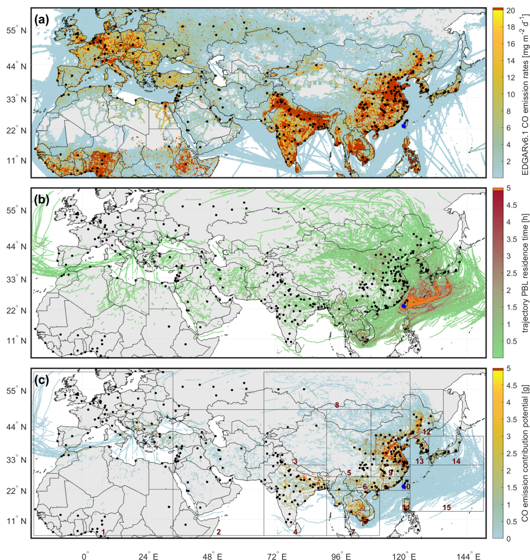
Figure 6. (a) EDGAR v6.1 CO emission rates from anthropogenic sources (March 2018), for clarity, not colour-coded below 0.01 \text{ mg m}^{-2} \text{ d}^{-1} ; (b) PBL residence time of air parcels (for flights AS-03 to AS-14) cumulated for a grid resolution of 0.1^\circ \times 0.1^\circ ; and (c) calculated CO emission uptake from PBL interpreted as emission contribution potential during EMERGE-Asia. Boxes in (c) mark selected study areas (summarised in Table 4, right-hand side). Black dots mark cities with more than one million inhabitants; the blue dot denotes the home base of HALO (Tainan Airport, Taiwan) during EMERGE-Asia.
