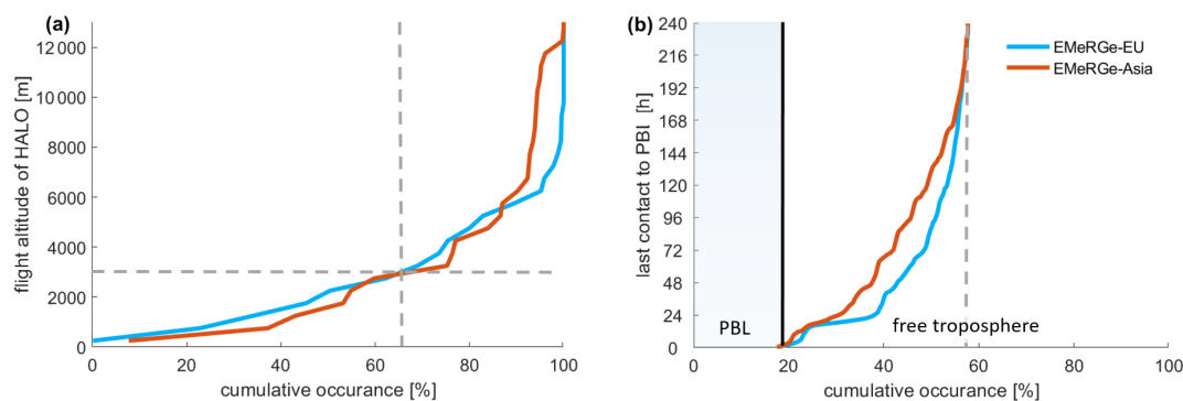
Figure 1. (a) Cumulative occurrences of HALO flight altitudes during EMeRGe and (b) last contact of probed air masses to planetary boundary layer (PBL) air, based on 10 d FLEXTRA back trajectories and ERA5 meteorological data.
