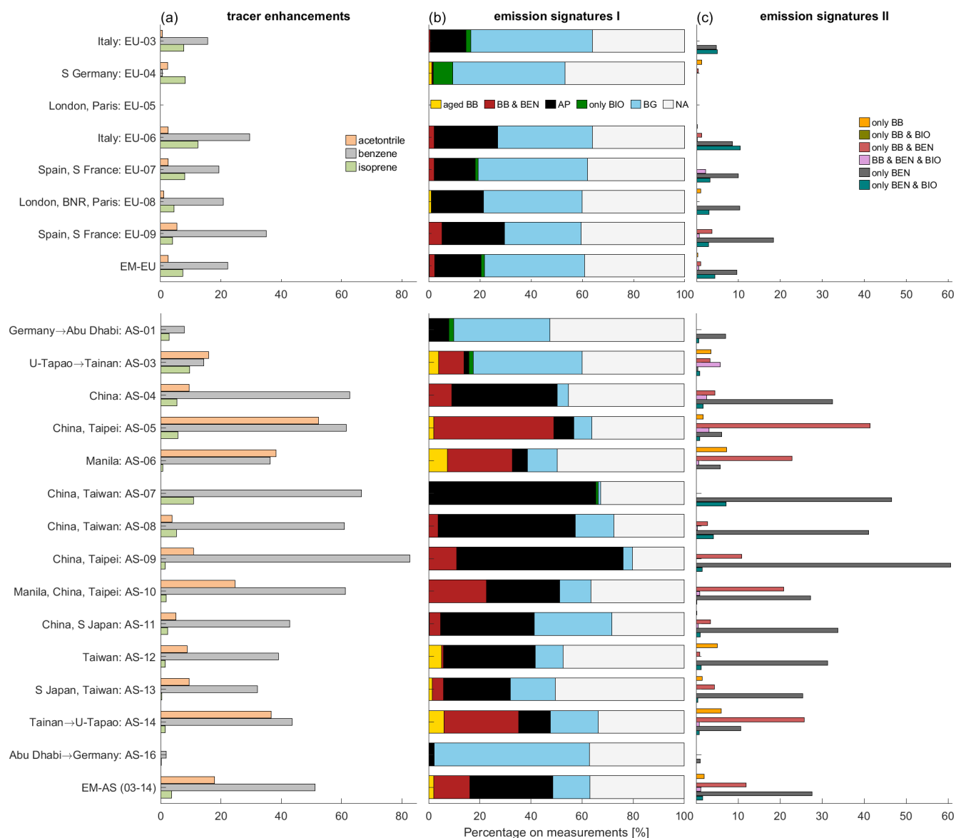
Figure 4. Fractions (%) of (a) enhancements over thresholds observed in acetonitrile, benzene and isoprene; (b) source signatures I (aged BB, BB & BEN and AP* inferred from observed enhancements only in acetonitrile and benzene and only BIO and BG* inferred with additional isoprene); and (c) source signatures II (inferred from observed enhancements in acetonitrile, benzene and isoprene). Top: EMeRGe-Europe, bottom: EMeRGe-Asia. EU-05 is not available due to instrument failure. The summary of EMeRGe-Asia excludes the non-Asian transfer flights AS-01 and AS-16. *AP – anthropogenic signatures, BB – biomass burning signatures, BEN – benzene enhancements, BIO – fresh biogenic signatures, BG – background, NA – not assessable during instrumental background detection and threshold transitions (due to PTR-MS measurement resolution of 1 min per tracer).
