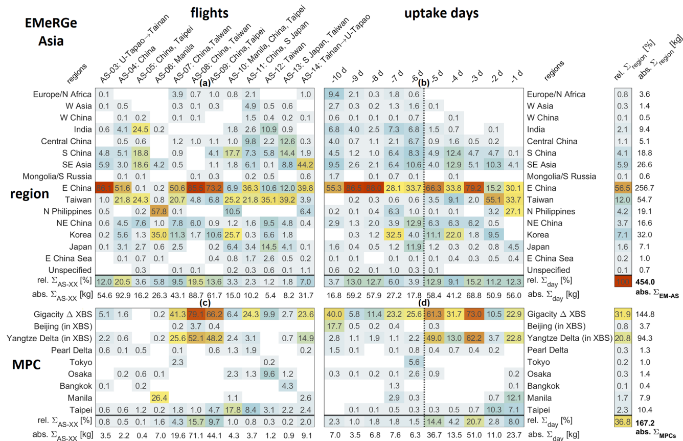
Figure 8. Absolute and relative CO contribution potentials of 15 source regions and nine MPCs (listed in Table 4) during EMeRGe-Asia. Absolute values (uncoloured rows) give the sum of contribution potentials for single flights ( \text{abs.} \sum_{AS-XX} ), uptake days ( \text{abs.} \sum_{day} ), as well as for source regions and MPCs ( \text{abs.} \sum_{region} ). For EMeRGe-Asia, the total uptake sum is 454.0 kg ( \text{abs.} \sum_{EM-AS} ) and for the selected MPCs 167.2 kg ( \text{abs.} \sum_{MPCs} ). Small deviations between absolute value sums and the total uptake sum are caused by rounding. Relative contribution potentials (colour-coded) of individual source regions are separated into contributing emission uptakes per flight ( a , c ), normalised to the absolute uptake sum per flight ( \text{region}_{AS-XX}/\text{abs.} \sum_{AS-XX} ), as well as separated into contributing emissions for the 10 particular uptake days prior to sampling with HALO ( b , d ), normalised to the absolute uptake sum per uptake day ( \text{region}_{day}/\text{abs.} \sum_{day} ). Relative uptake sums \text{rel.} \sum_x are normalised to the total uptake sum ( \text{rel.} \sum_x = \text{abs.} \sum_x / \sum_{EM-AS} , with x = AS-XX , day and region). Target regions are given in the column label after flight labels. Regions are sorted by location from west (top) to east (bottom). Unspecified includes all areas outside the selected regions. XBS – Xian–Beijing–Shanghai.
