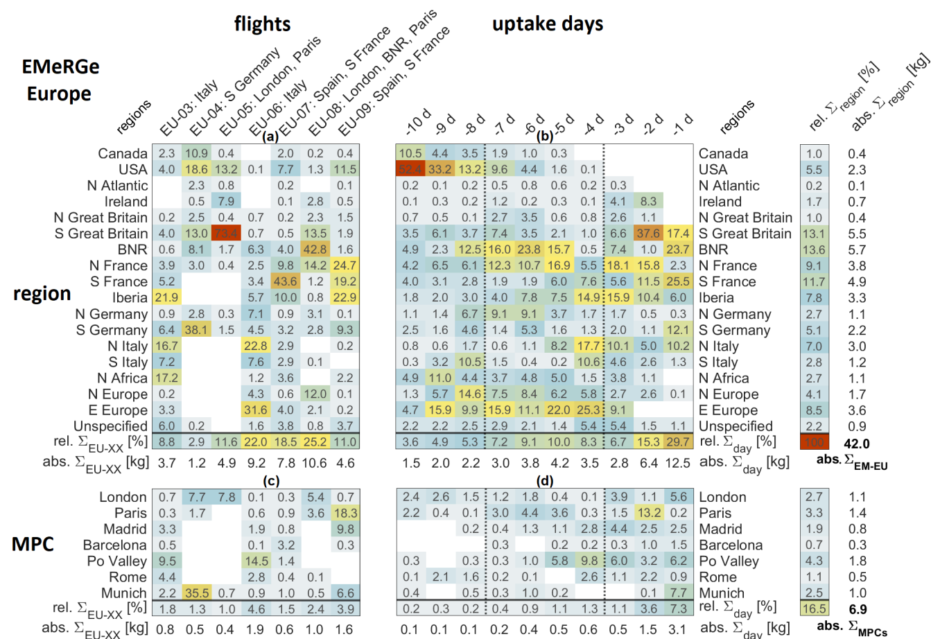
Figure 7. Absolute and relative CO contribution potentials of 17 source regions and seven MPCs (listed in Table 4) during EMERGE-Europe. Absolute values (uncoloured rows) give the sum of contribution potentials for single flights ( \text{abs.} \Sigma_{EU-XX} ), uptake days ( \text{abs.} \Sigma_{day} ), as well as for source regions and MPCs ( \text{abs.} \Sigma_{region} ). For EMERGE-Europe, the total uptake sum is 42.0 kg ( \text{abs.} \Sigma_{EM-EU} ) and for the selected MPCs 6.9 kg ( \text{abs.} \Sigma_{MPC} ). Small deviations between absolute value sums and the total uptake sum are caused by rounding. Relative contribution potentials (colour-coded) of individual source regions are separated into contributing emission uptakes per flight (a, c), normalised to the absolute uptake sum per flight ( \text{region}_{EU-XX} / \text{abs.} \Sigma_{EU-XX} ), as well as separated into contributing emissions for the 10 particular uptake days prior to sampling with HALO (b, d), normalised to the absolute uptake sum per uptake day ( \text{region}_{day} / \text{abs.} \Sigma_{day} ). Relative uptake sums \text{rel.} \Sigma_x are normalised to the total uptake sum ( \text{rel.} \Sigma_x = \text{abs.} \Sigma_x / \Sigma_{EM-EU} , with x = EU-XX , day and region). Target regions are given in the column label after flight labels. Regions are sorted by location from west (top) to east (bottom). Unspecified includes all areas outside the selected regions.
