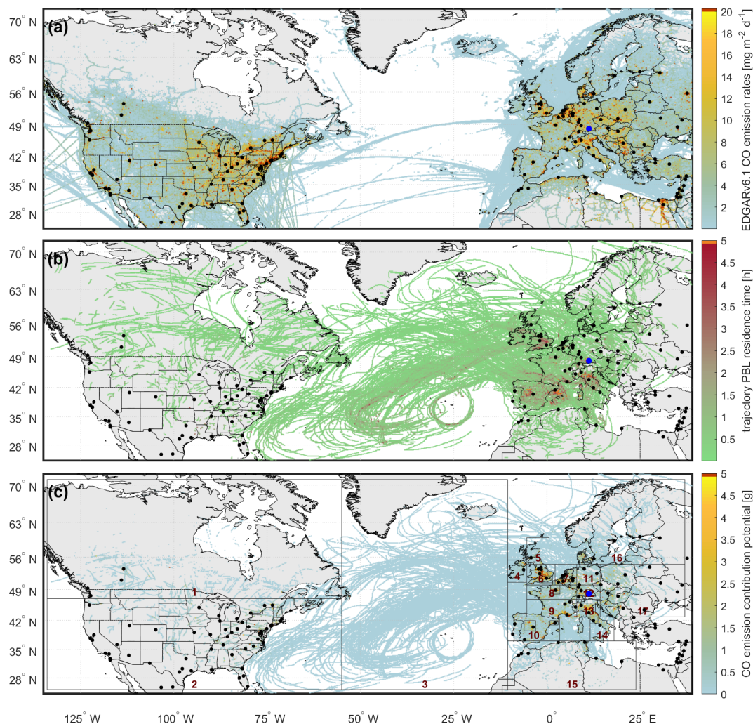
Figure 5. (a) EDGAR v6.1 CO emission rates from anthropogenic sources (July 2018), for clarity, not colour-coded below 0.01 \text{ mg m}^{-2} \text{ d}^{-1} ; (b) PBL residence time of air parcels cumulated for a grid resolution of 0.1^\circ \times 0.1^\circ ; and (c) modelled CO emission uptake from the PBL interpreted as emission contribution potential during EMeRGe-Europe. Boxes in (c) mark selected study areas (summarised in Table 4, left). Black dots mark cities with more than one million inhabitants; the blue dot denotes the home base of HALO (Oberpfaffenhofen Airport near Munich, Germany) during EMeRGe-Europe.
