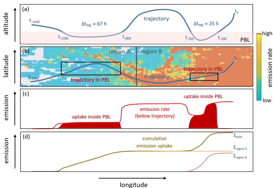
Figure 3. Graphical representation (simplified example) of our Lagrangian CO uptake model based on the PBL height and trajectory pathways, with longitude as x axis. (a) Trajectory altitude. An example trajectory (sampled by the aircraft at time t_0 ) enters the PBL for two different periods, between t_{-1200} and t_{-800} , as well as between t_{-250} and t_{-100} ( t_{-100} means 100 backward calculation steps = 1000 min = 16.7 h). During these periods, CO is taken up, that is, the trajectory is loaded with CO emitted on the ground. (b) Geographic map. CO emission rates from EDGAR (shaded) with a trajectory (blue line) and rectangles in which the trajectory descends into the PBL. Exemplary, two example regions A and B are defined. (c) Time series. Emission rate along the trajectory (red line) and CO uptake periods (filled red regions) along the trajectory. (d) Total and subtotal (region A and B) cumulative CO uptake (dark yellow line) along the trajectory.
