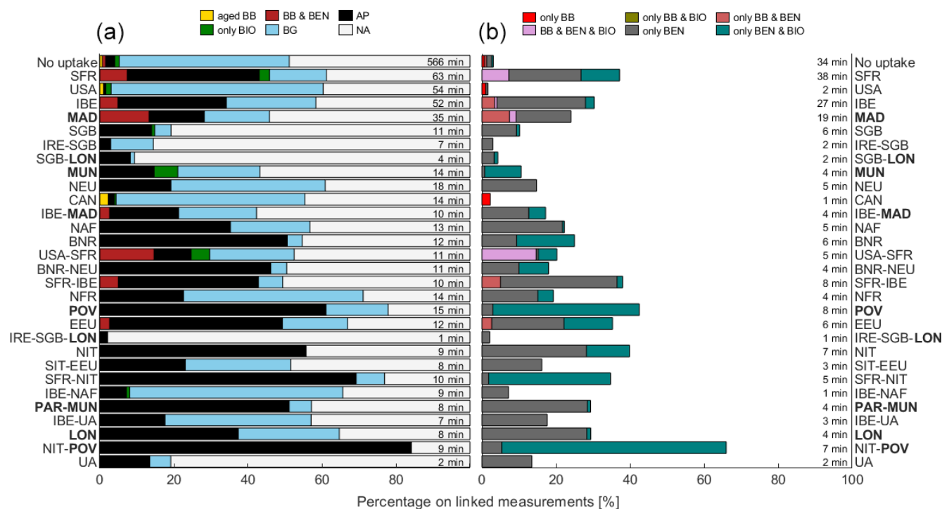
Figure 10. Source signatures (I – left and II – right, using the tracers acetoneitrile, benzene and isoprene) of contributing regions as chemical fingerprints during EMeRGe-Europe. The temporal contribution of identified signatures to the measurements is shown on the right-hand side of the bars and differ from signatures I to II due to the usage of two and three tracers, respectively. For full names of source regions see Table 4. For abbreviations of source signatures see caption in Fig. 4.
