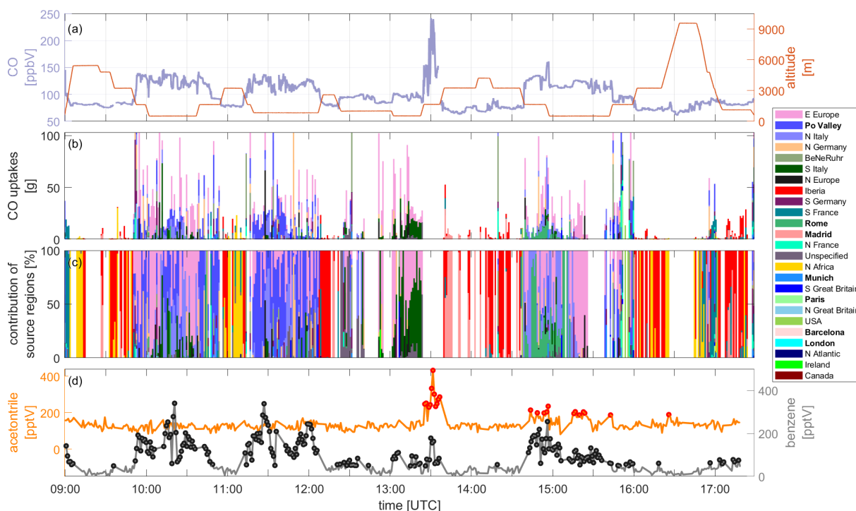
Figure 9. Time series of modelled source-region-specific CO uptakes and measured CO, acetonitrile and benzene for the EMERGE-Europe flight EU-06, 20 July 2017, targeting Italian outflows. (a) CO measurements and flight altitude, (b) modelled CO uptake sums along 10 d back trajectories colour-coded by originating source regions (sorted by total flight uptake sums – top to bottom, MPCs in bold), (c) relative contribution of source regions on CO uptake sums, and (d) acetonitrile and benzene measurements with colour-coded tracer enhancements over defined threshold (red and black dots, respectively).
