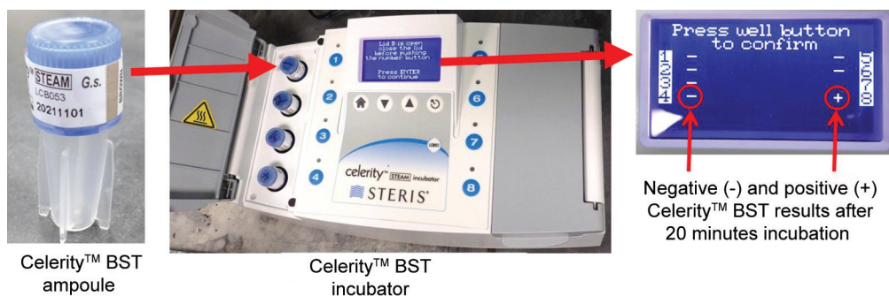
Fig. 1: Celerity™ BST system
