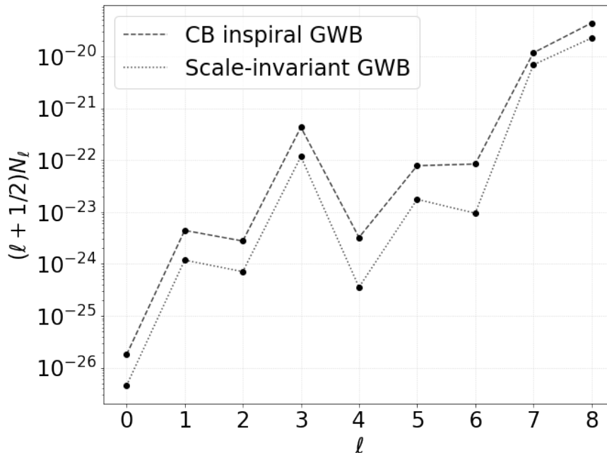
Figure 13. Noise power spectrum for LISA in \Omega_{\text{GW}}^2 units at reference frequency f_0 = 0.01 Hz. Note the \mathcal{N}_\ell here is in good agreement with the curve shown in [208], figure 4, taking into account that the observation time considered here is one year, whereas in [208] it is four.
