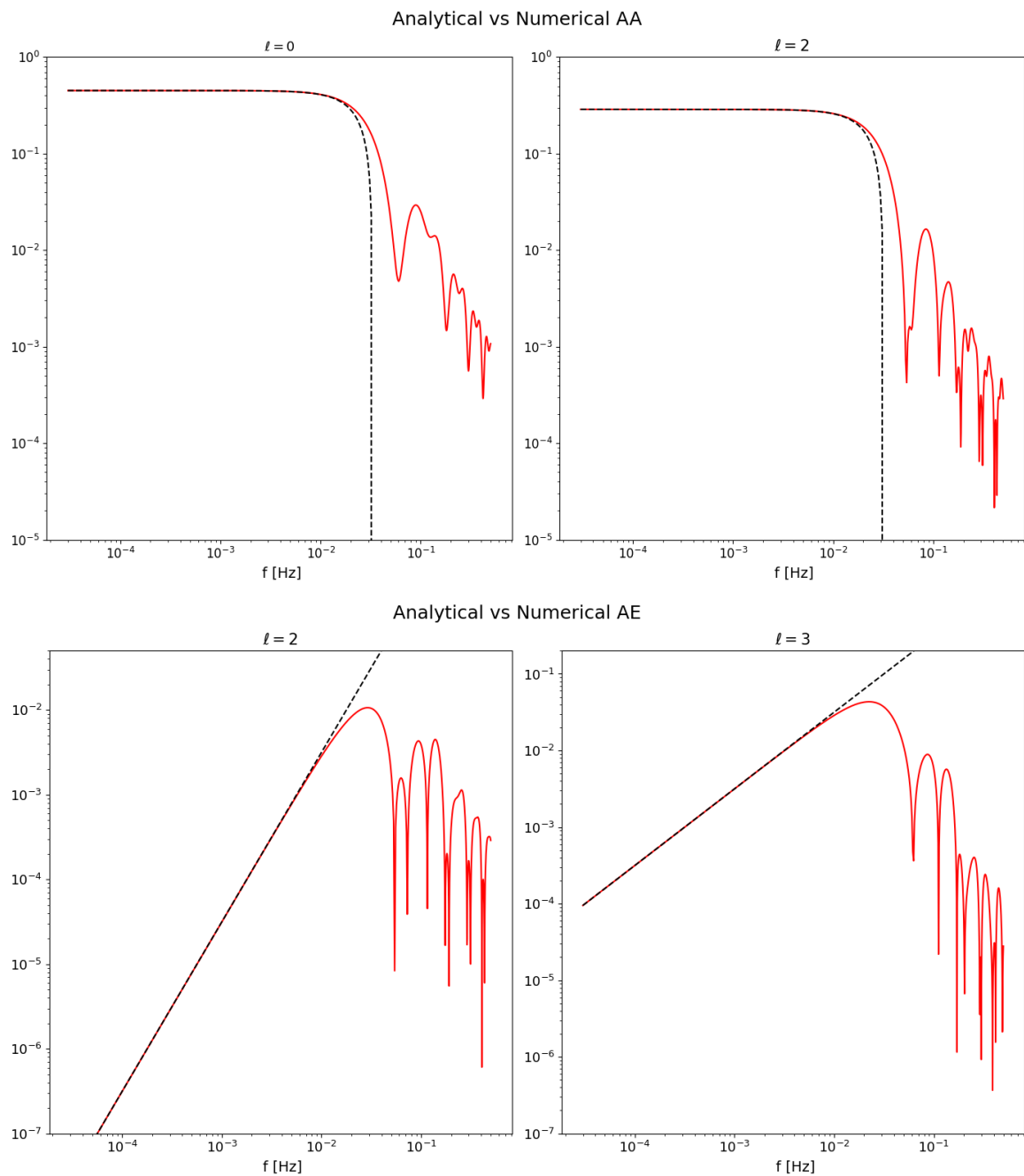
Figure 7. Angular overlap functions, defined through eqs. (4.15) and (4.23), for the first few multipoles for the AA = EE correlation (first row) and for the AE correlation (second row). The solid red line is from an exact evaluation. The dashed black line is the small frequency approximation in table 1.
