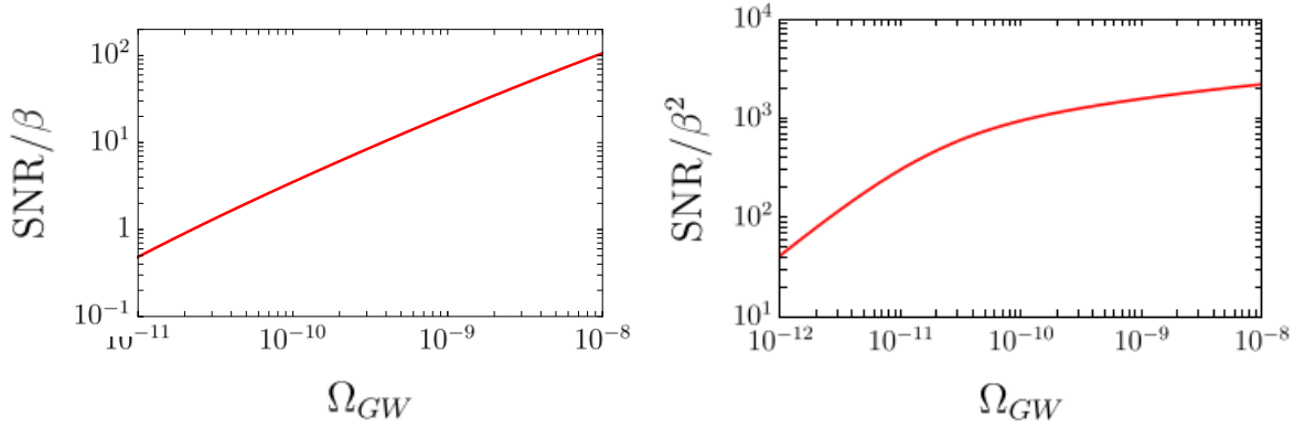
Figure 10. The SNR for the dipole (left) and the quadrupole (right) induced by boosting an isotropic SGWB with fractional energy density \Omega_{GW} , assumed to be scale free across the LISA band. An observation time of T = 1 year is assumed.
