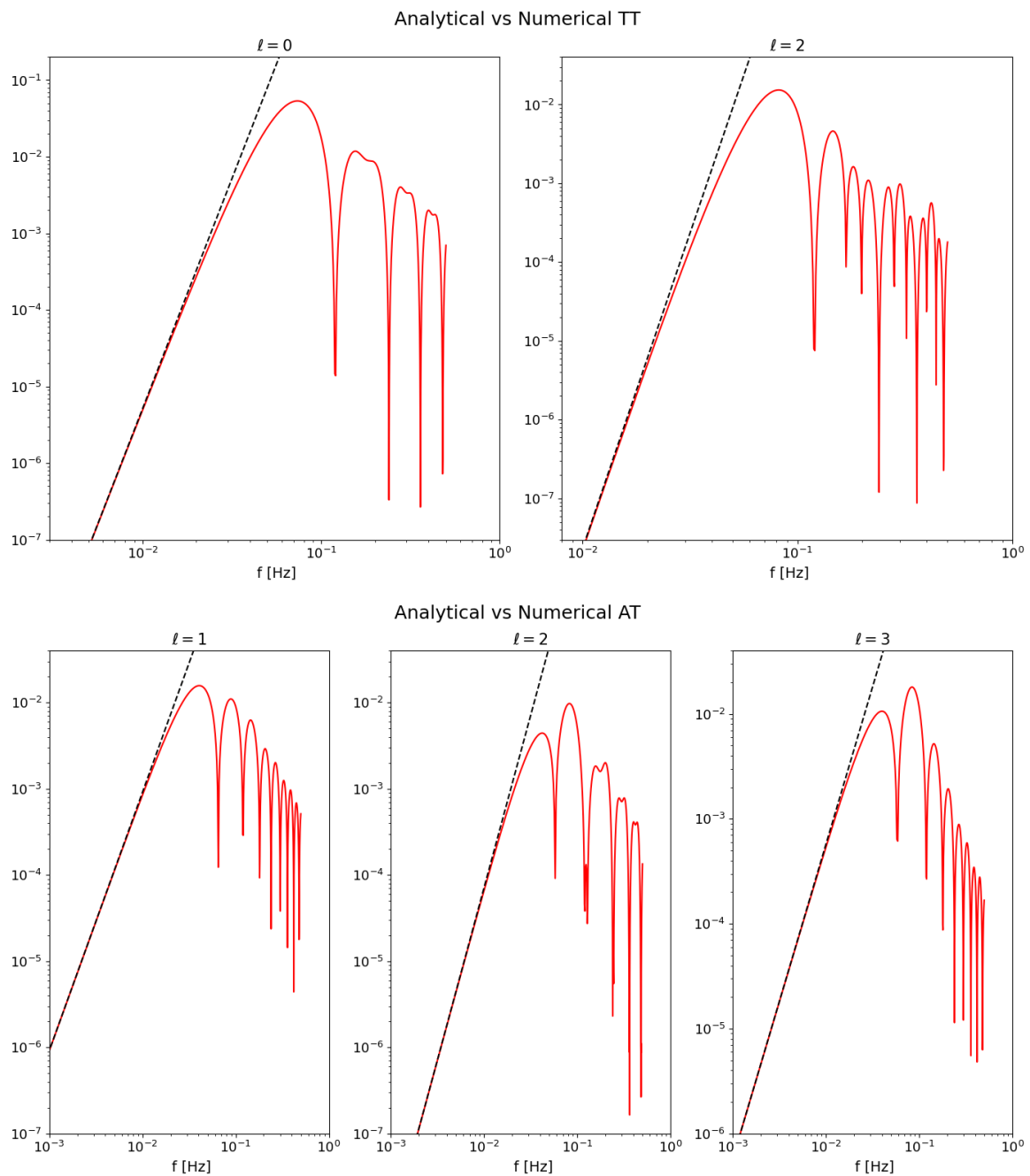
Figure 8. Angular overlap functions, defined through eqs. (4.15) and (4.23), for the first few multipoles for the TT correlation (first row) and for the AT = ET correlation (second row). The solid red line is from an exact evaluation. The dashed black line is the small frequency approximation in table 1.
