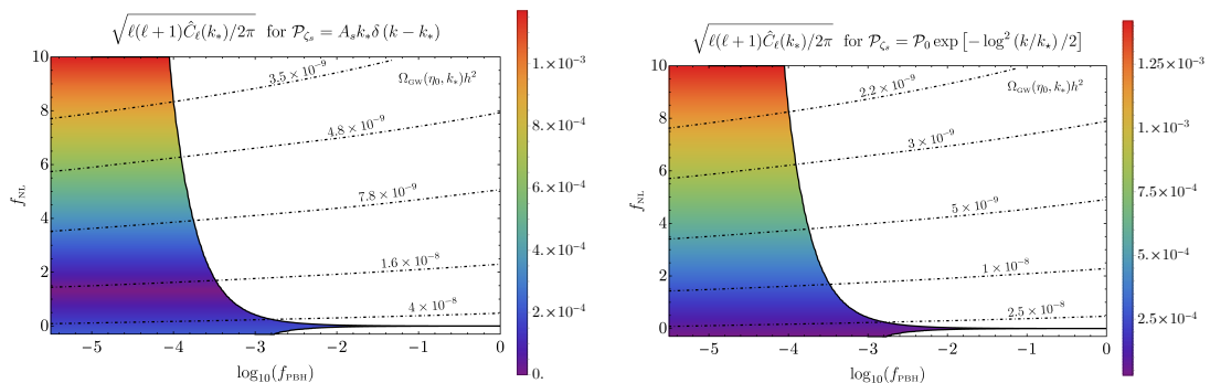
Figure 4. Contour plot of the GW anisotropy in the parameter space of f_{\text{PBH}} and f_{\text{NL}} allowed by the Planck constraints for a monochromatic (left) and lognormal (right) power spectrum at small scales. We fixed the SGWB characteristic scale around the maximum sensitivity of LISA. The dot-dashed lines identify the corresponding present day GWs abundance. Figure taken from ref. [101] (with \hat{C}_\ell(k_*) corresponding to our C_\ell^{\text{GW}} ).
