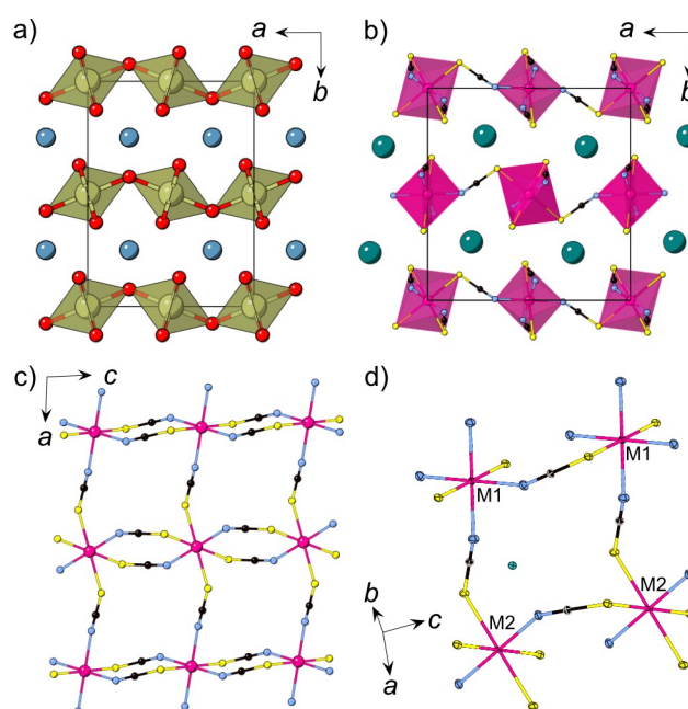
Fig. 1 a) The structure of CaIrO 3 with iridium polyhedra connected via corner-sharing ( a axis) and edge-sharing ( c axis) [IrO 6 ] octahedra, Ca = blue, Ir = brown, O = red. b) Crystal structure of CsMn(NCS) 3 at 120 K obtained from single crystal X-ray diffraction. c) A single [Mn(NCS) 3 ] - layer. d) Close-up view of the structure highlighting the two chemically independent metal ions (M1, M2). Cs = green, Mn = pink, N = blue, C = black, S = yellow.
