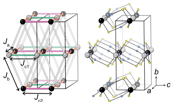
Fig. 5 The four nearest-neighbour magnetic interactions in \text{CsM}(\text{NCS})_3 . M1 and M2 are grey and black respectively and the thiocyanate ligands are represented with sulfur (yellow) and nitrogen (blue) atoms only. Caesium cations and carbon atoms have been removed for clarity.
