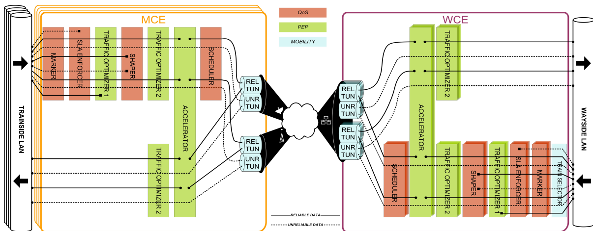
Fig. 2. General architecture – data plane
