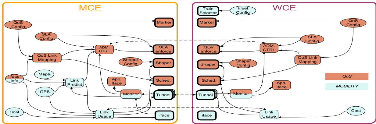
Fig. 1. General architecture – control plane
