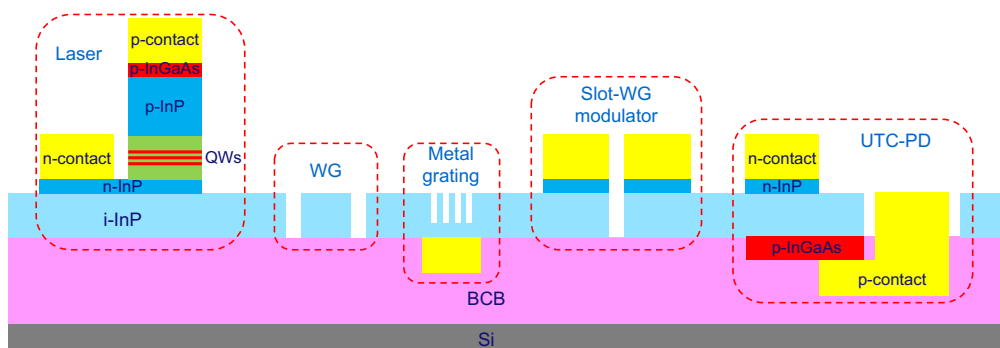
Fig. 2. A new integration platform based on double-sided processing.
