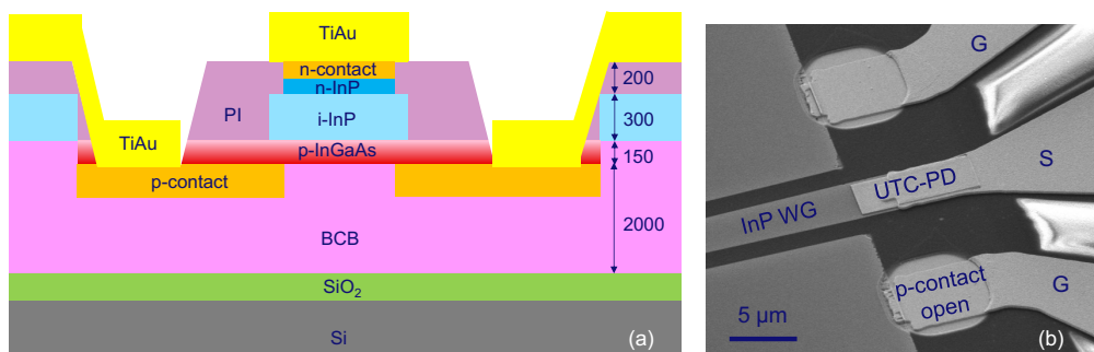
Fig. 1. (a) Cross-section of the UTC-PD. Thickness in nm. (b) SEM photo of the device.
