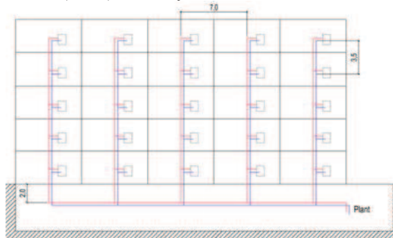
Figure 1: Building and distribution network scheme
