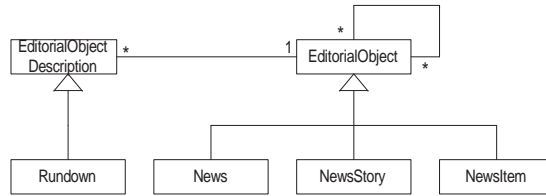
Fig. 3. The EditorialObject class, with subclasses News , NewsStory , and NewsItem , and associated Rundown description class.
