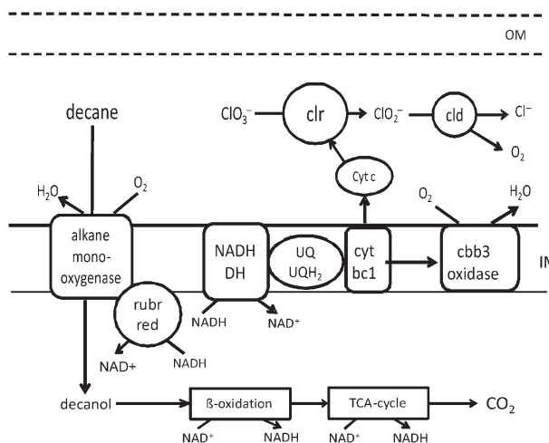
Fig. 1. Proposed model of anaerobic n -decane degradation. After reduction of chlorate by chlorate reductase the resulting chlorite is decomposed into chloride ions and molecular oxygen. Under anaerobic conditions, the produced oxygen can be used by alkane-1-monooxygenase to oxidize decane to decanol. OM, outer membrane; IM, Inner membrane; clr, chlorate reductase; cld, chlorite dismutase; Cyt C, 8.6 kDa periplasmic cytochrome; cbb3 oxidase, cbb3-type cytochrome c oxidase; UQ/UQH 2 , ubiquinone/ubihydroxyquinone; rubr/red, rubredoxin and rubredoxin reductase, which in P. chloritidismutans AW-1 T are fused into a single protein.
