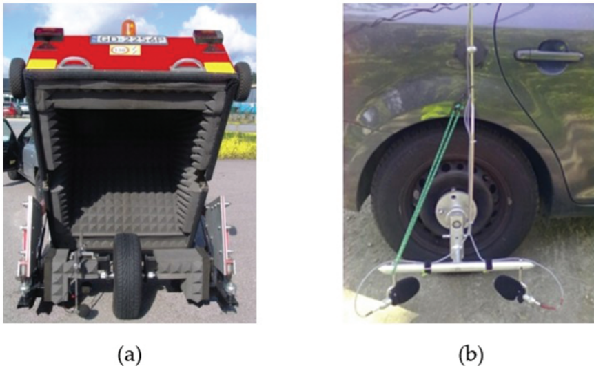
Figure 2. Examples of CPX devices: at left (a) the interior of the TUG Tiresonic Mk4 CPX trailer [28]; at right (b) the University of Minho device [14].
