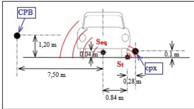
Figure 5. Noise sources location [38].
