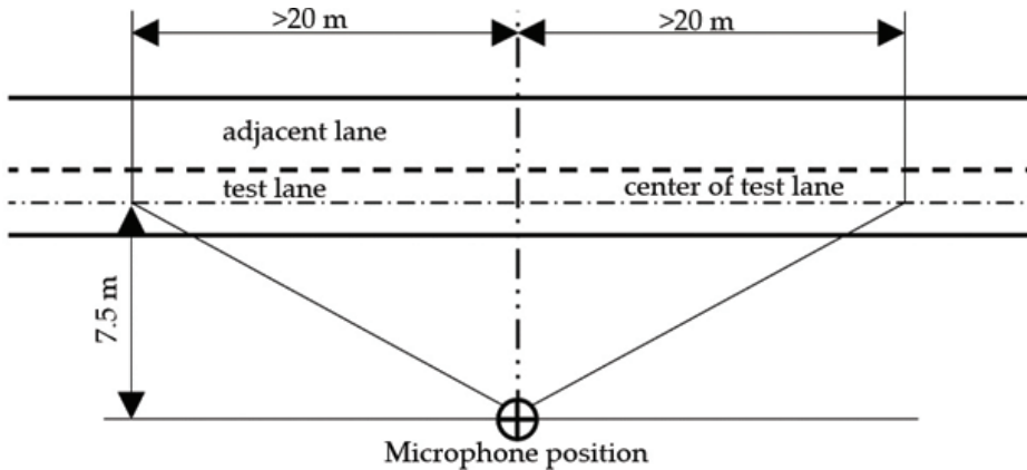
Figure 1. SPB testing geometry.
