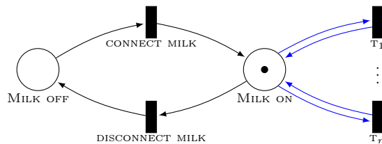
Fig. 13: Encoding a feature selection as a Petri net marking.
