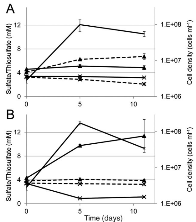
Fig. 2. Oxidation of thiosulfate during growth of Aeropyrum pernix with either oxygen (A) or perchlorate (B). Primary y-axis shows thiosulfate (crosses) and sulfate concentrations (triangles); cell densities (solid lines/no symbols) are plotted against secondary y-axis. Dashed lines indicate change of respective sulfur compounds in (uninoculated) chemical controls. Perchlorate and oxygen concentrations are not displayed. Means ( n = 2 ) \pm range (bars). Note that the expected stoichiometry where 2 chlorite molecules react with 1 thiosulfate molecule to form 2 sulfate molecules (Fig. 3) was roughly met in the experiment [all available perchlorate (7.9 mM) was depleted after 5 days]. Also, the activity of the cultures in Fig. 2 was higher compared with that in Fig. 1.
