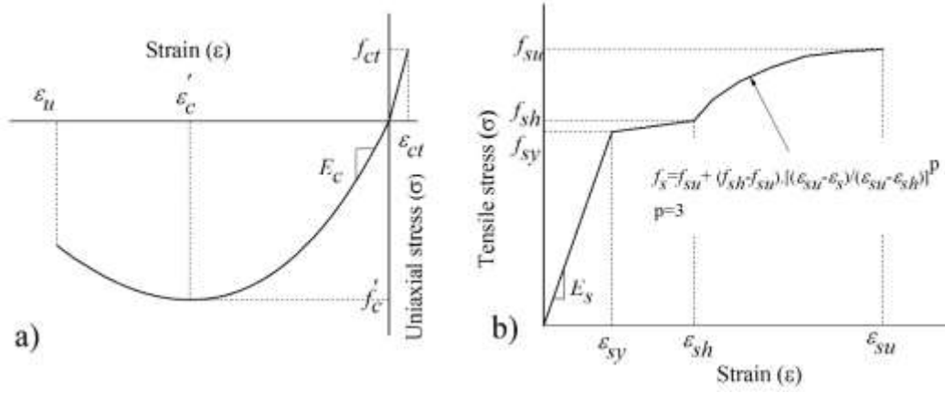
Figure 12: Stress-strain relationship used in DOCROS to simulate: a) concrete, b) steel bars
