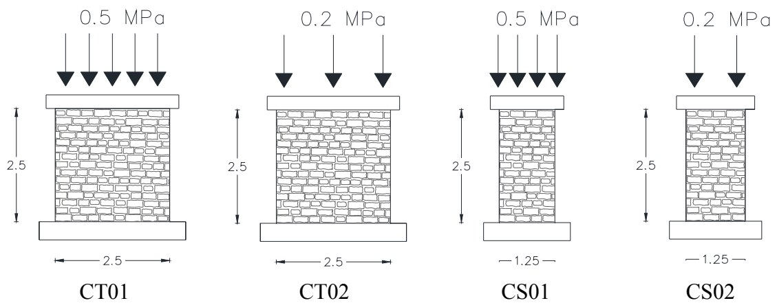
Figure 2: Panels for the in-plane cyclic shear tests.
